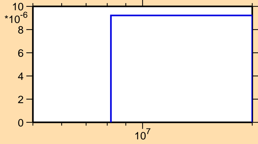
\sigma vs. E for ^{163}\text{Gd}(n,t)
