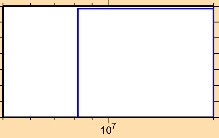
\sigma vs. E for ^{163}\text{Gd}(n,\text{nd})
