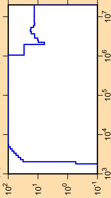
\Delta\mu/\mu vs. E for ^{164}\text{Gd}(\text{mt251})
