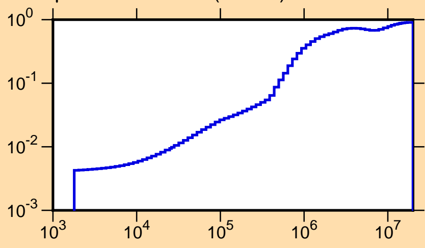
\mu vs. E for ^{164}\text{Gd}(\text{mt251})
