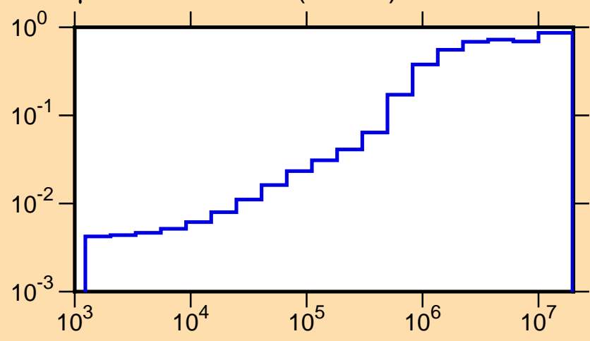
\mu vs. E for ^{164}\text{Gd}(\text{mt251})
