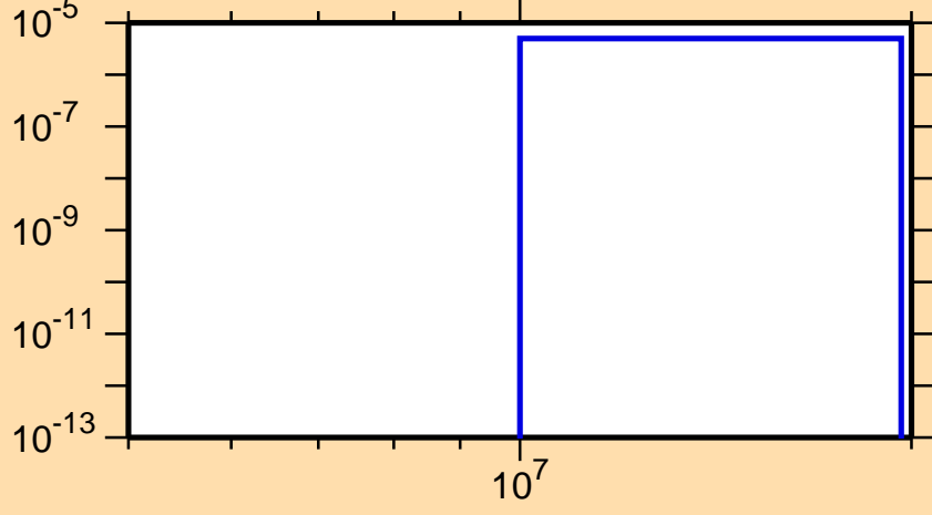
\sigma vs. E for ^{164}\text{Gd}(n,t)
