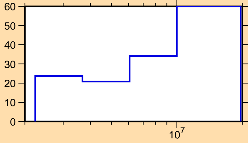
\Delta\sigma/\sigma vs. E for ^{164}\text{Gd}(n,inel.)
