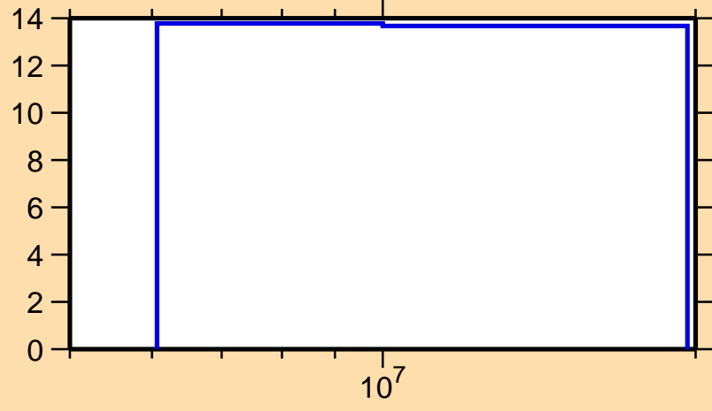
\Delta\sigma/\sigma vs. E for ^{164}\text{Gd}(n,el.)
