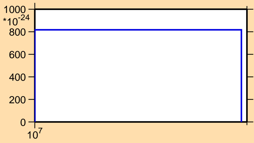
\sigma vs. E for ^{164}\text{Gd} (mt 11)
