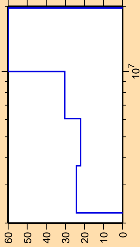
\Delta\sigma/\sigma vs. E for ^{164}\text{Gd}(n,ncont.)
