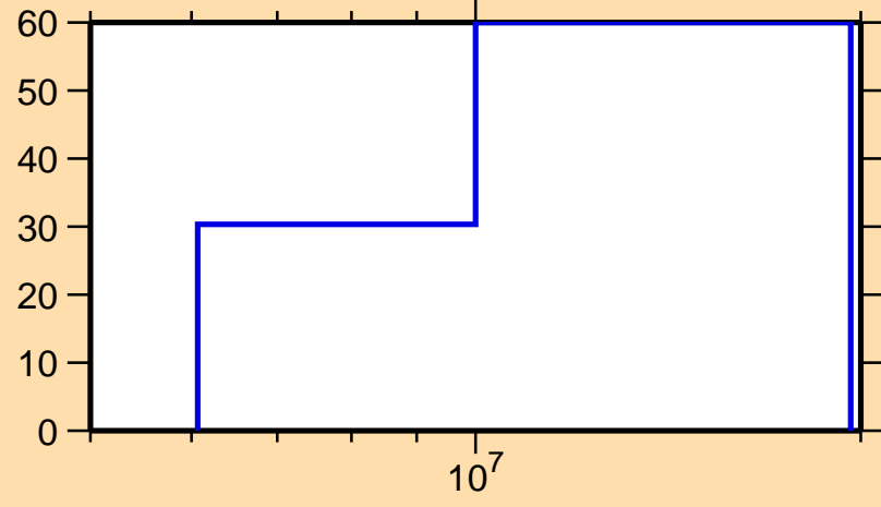
\Delta\sigma/\sigma vs. E for ^{164}\text{Gd}(n,ncont.)
