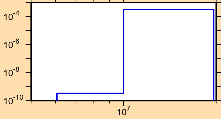
\sigma vs. E for ^{164}\text{Gd}(n,p)
