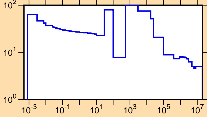
\sigma vs. E for ^{164}\text{Gd}(n,\text{tot.})
