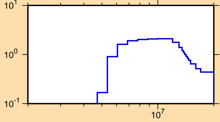
\sigma vs. E for ^{165}\text{Gd}(n,2n)
