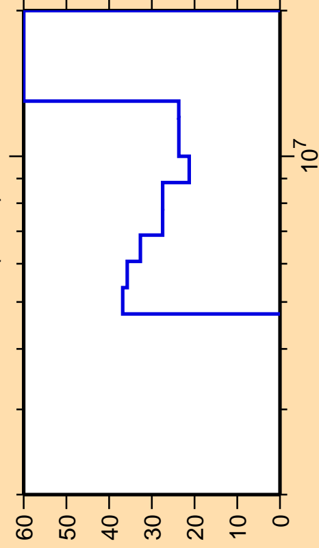
\Delta\sigma/\sigma vs. E for ^{165}\text{Gd}(n,2n)
