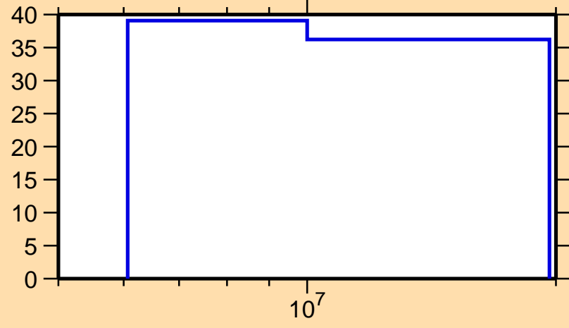
\Delta\sigma/\sigma vs. E for ^{165}\text{Gd}(n,el.)
