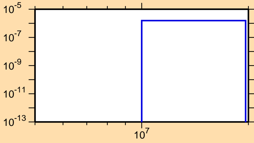
\sigma vs. E for ^{165}\text{Gd}(n,n\alpha)
