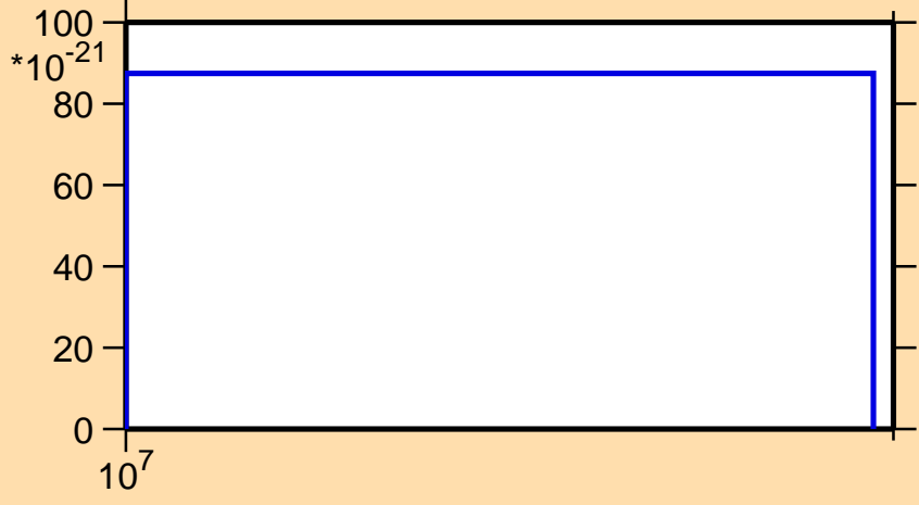
\sigma vs. E for ^{165}\text{Gd} (mt 11)
