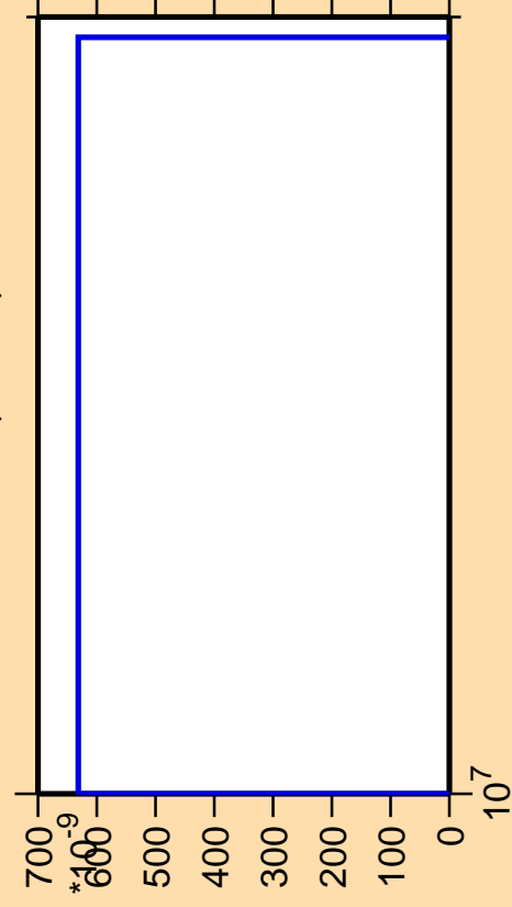
\Delta\sigma/\sigma vs. E for ^{165}\text{Gd} (mt 11)
