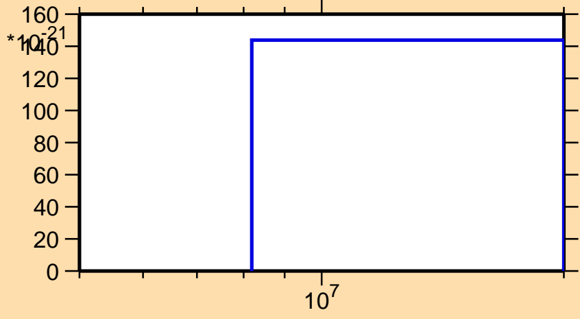
\sigma vs. E for ^{165}\text{Gd}(\text{mt } 11)
