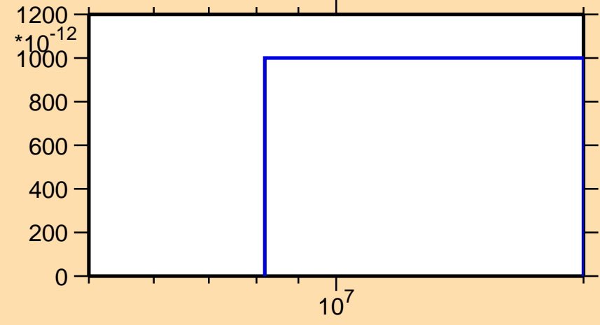
\sigma vs. E for ^{165}\text{Gd}(n,nd)
