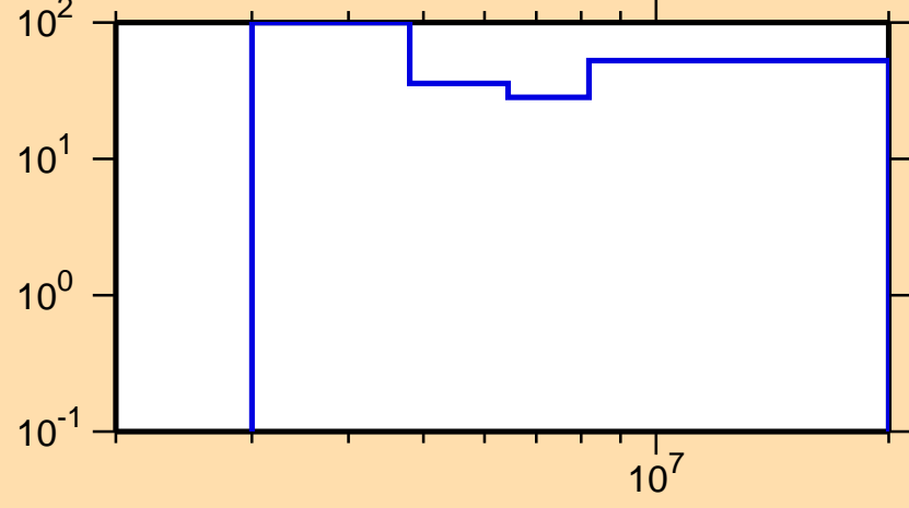
\Delta\sigma/\sigma vs. E for ^{165}\text{Gd}(n,2n)
