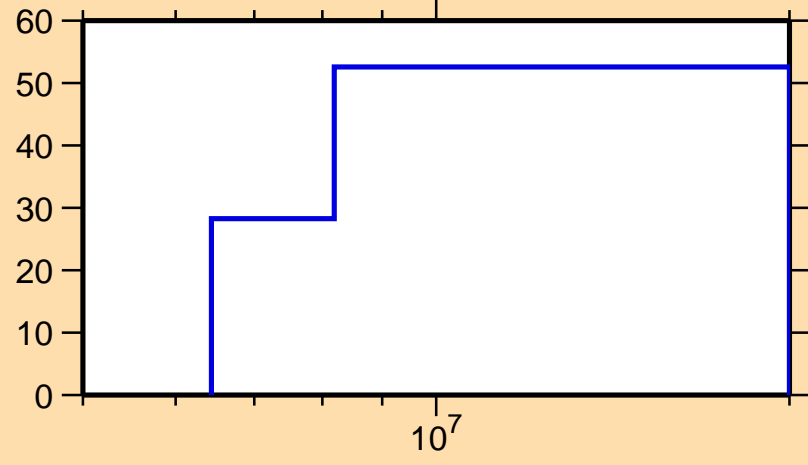
\Delta\sigma/\sigma vs. E for ^{165}\text{Gd}(n,2n)
