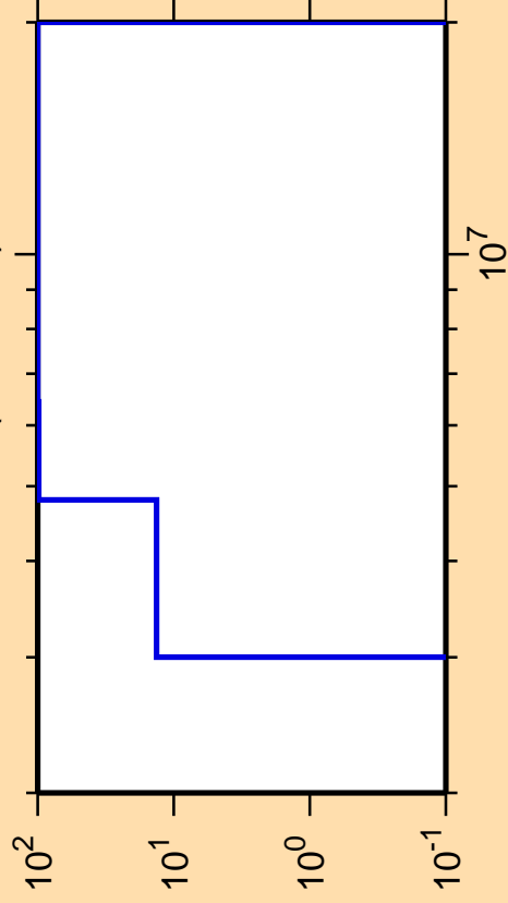
\Delta\sigma/\sigma vs. E for ^{165}\text{Gd}(n,n_{\text{cont}})
