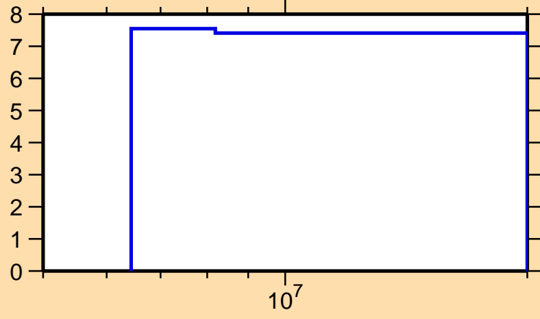
\Delta\sigma/\sigma vs. E for ^{165}\text{Gd}(n,\text{nonel.})
