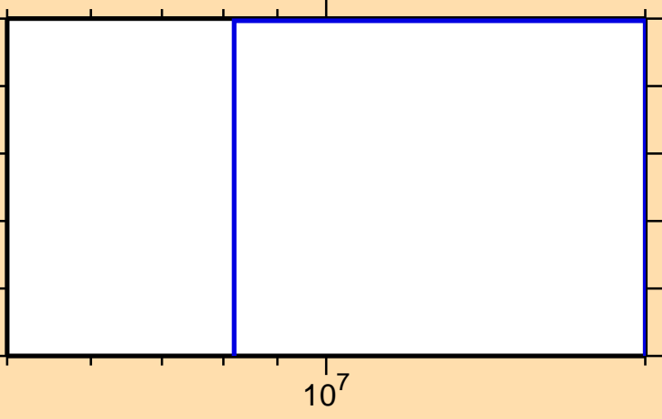
\sigma vs. E for ^{165}\text{Gd}(n,2n\alpha)
