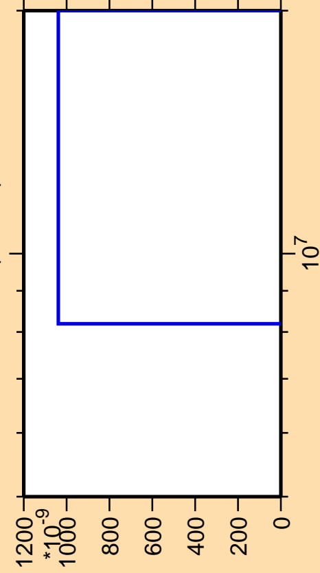
\Delta\sigma/\sigma vs. E for ^{165}\text{Gd}(\text{mt } 11)
