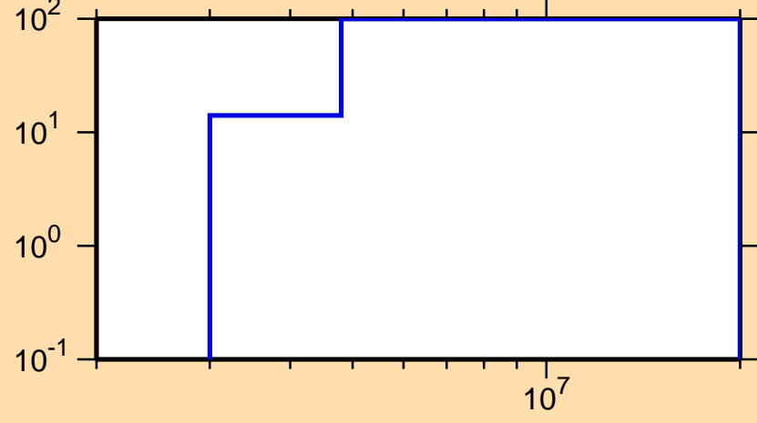
\Delta\sigma/\sigma vs. E for ^{165}\text{Gd}(n,\text{inel.})
