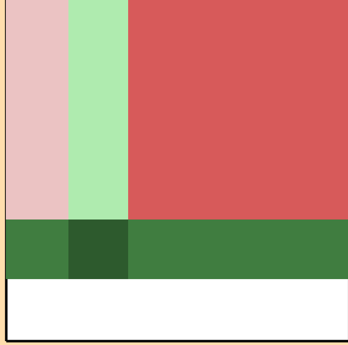
\Delta\sigma/\sigma vs. E for ^{165}\text{Gd}(n,\text{tot.})
