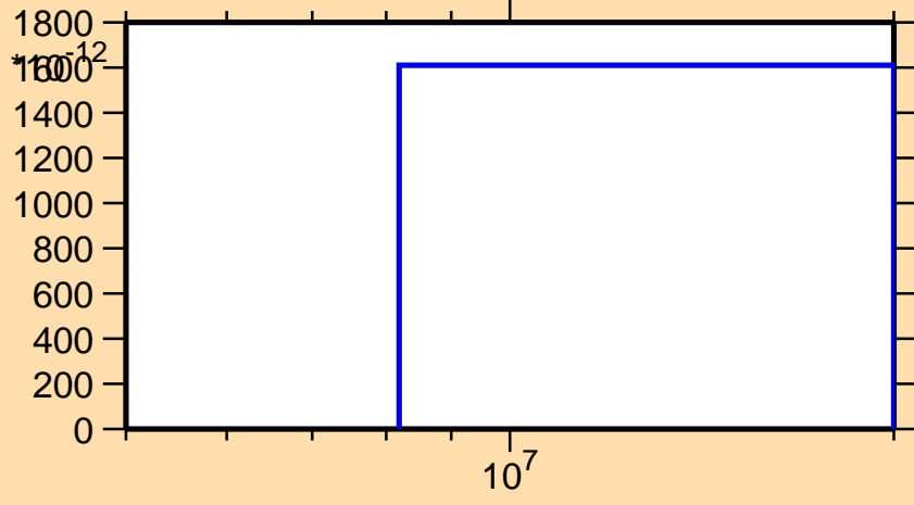
\sigma vs. E for ^{165}\text{Gd}(n,nt)
