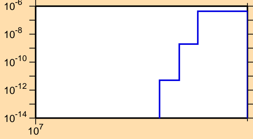
\sigma vs. E for ^{167}\text{Gd}(n,nt)
