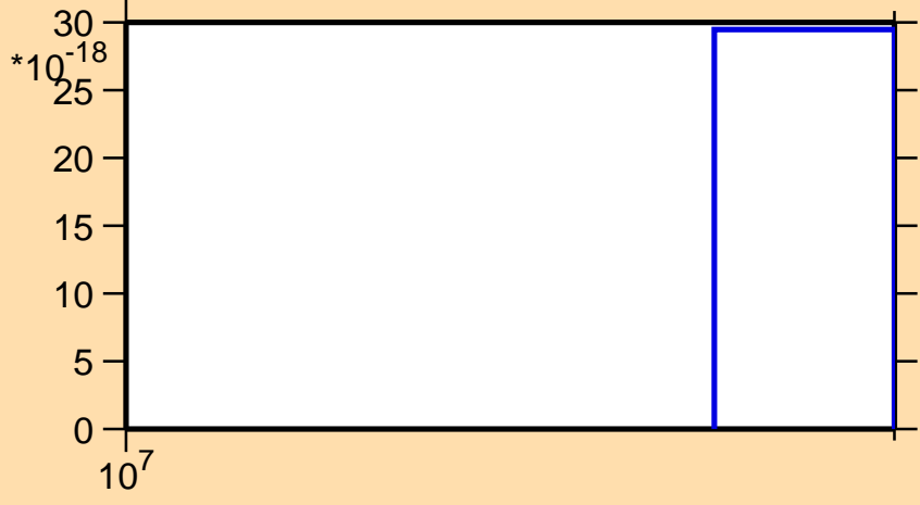
\sigma vs. E for ^{167}\text{Gd}(\text{mt } 11)
