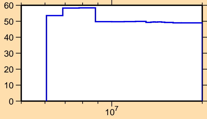
\Delta\sigma/\sigma vs. E for ^{167}\text{Gd}(n,ncont.)
