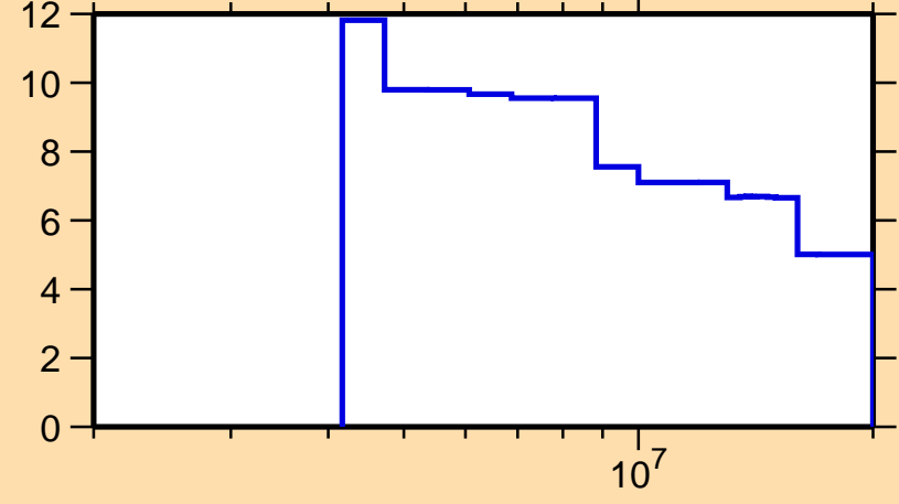
\Delta\sigma/\sigma vs. E for ^{167}\text{Gd}(n,\text{nonel.})
