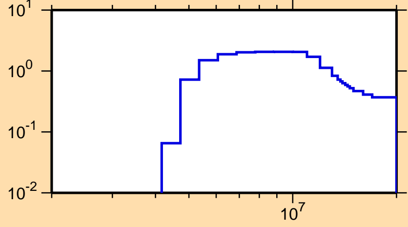
\sigma vs. E for ^{167}\text{Gd}(n,2n)
