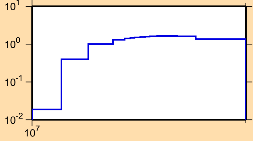
\sigma vs. E for ^{167}\text{Gd}(n,3n)
