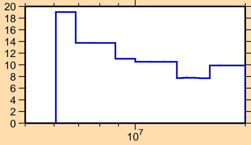
\Delta\sigma/\sigma vs. E for ^{167}\text{Gd}(n,\text{el.})
