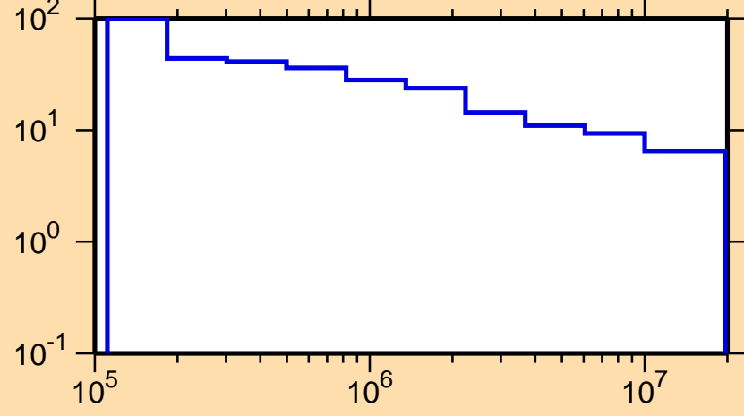
\Delta\sigma/\sigma vs. E for ^{167}\text{Gd}(n,\text{nonel.})
