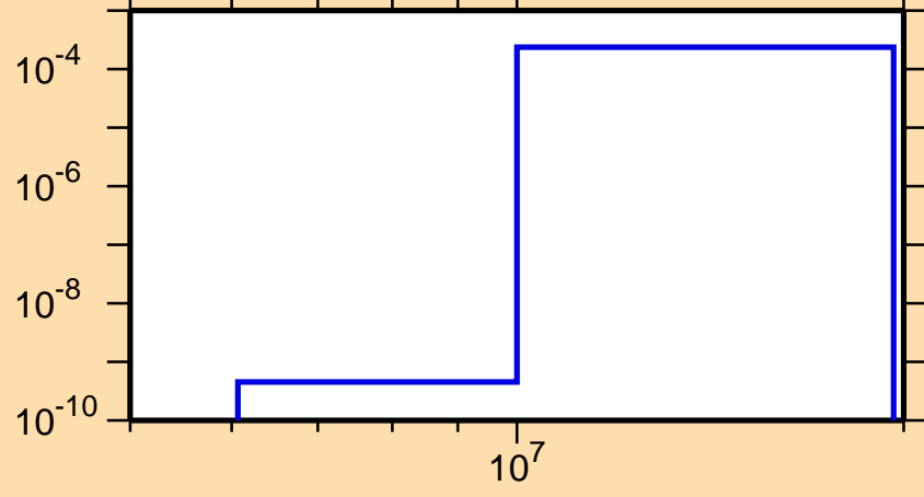
\sigma vs. E for ^{167}\text{Gd}(n,p)
