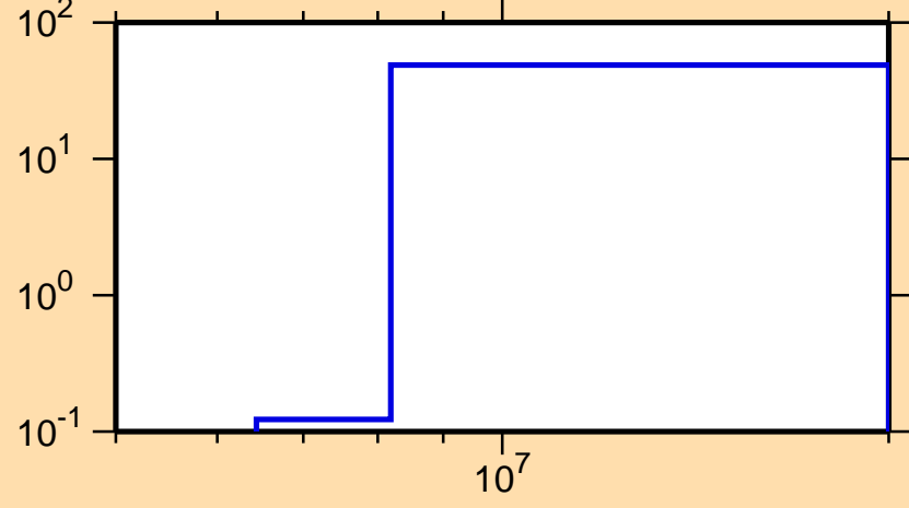
\Delta\sigma/\sigma vs. E for ^{167}\text{Gd}(n,p)
