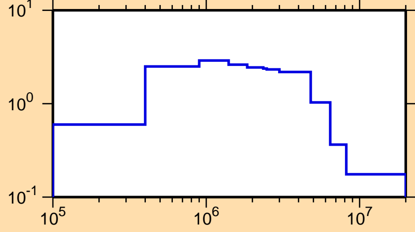
\sigma vs. E for ^{167}\text{Gd}(n,\text{inel.})
