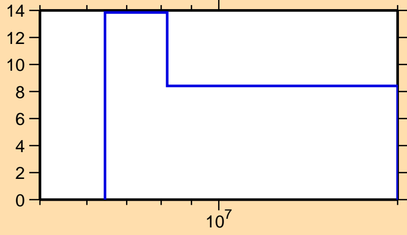
\Delta\sigma/\sigma vs. E for ^{167}\text{Gd}(n,el.)
