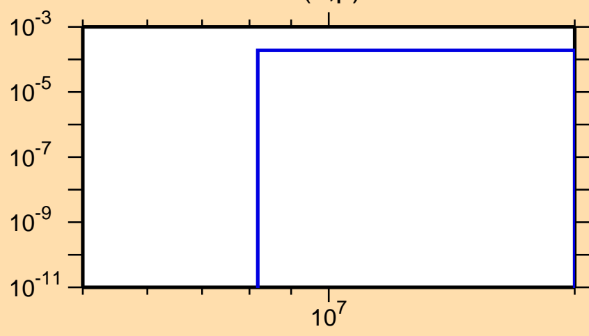
\sigma vs. E for ^{167}\text{Gd}(n,p)
