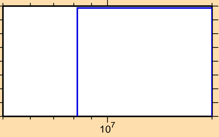
\sigma vs. E for ^{167}\text{Gd}(n,np)
