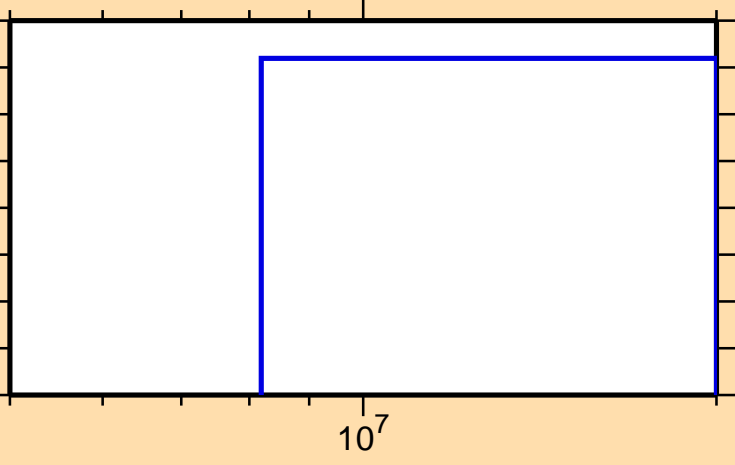
\sigma vs. E for ^{167}\text{Gd}(n,nt)
