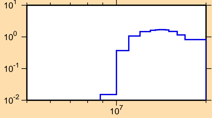
\sigma vs. E for ^{169}\text{Gd}(n,3n)
