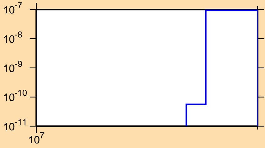
\sigma vs. E for ^{169}\text{Gd}(n,\text{nd})
