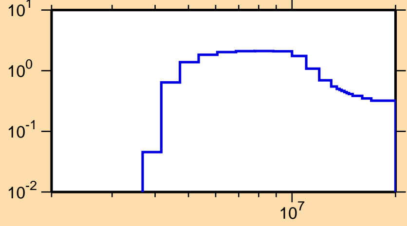
\sigma vs. E for ^{169}\text{Gd}(n,2n)
