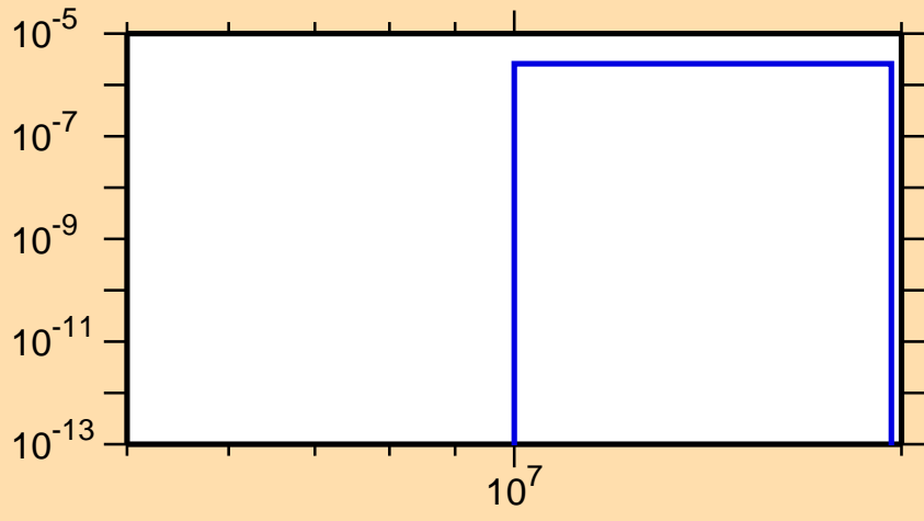
\sigma vs. E for ^{169}\text{Gd}(n,d)
