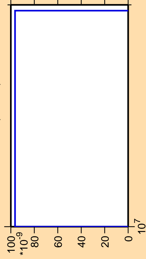
\Delta\sigma/\sigma vs. E for ^{169}\text{Gd} (mt 11)
