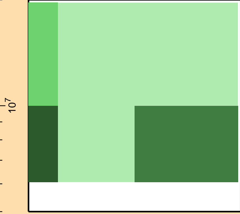
\Delta\sigma/\sigma vs. E for ^{169}\text{Gd}(n,n_1)
