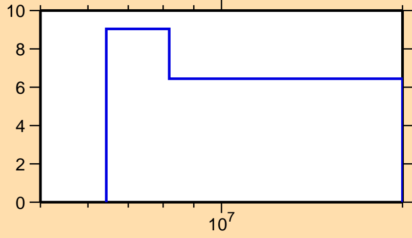
\Delta\sigma/\sigma vs. E for ^{169}\text{Gd}(n,\text{tot.})
