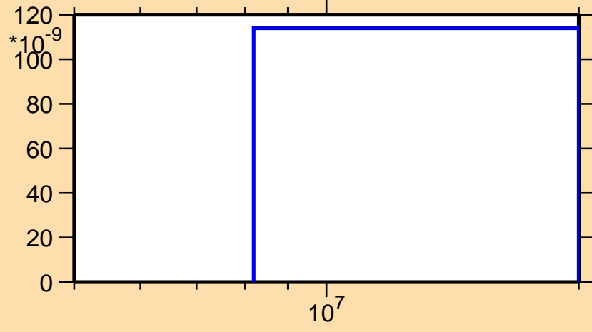
\sigma vs. E for ^{169}\text{Gd}(n,np)
