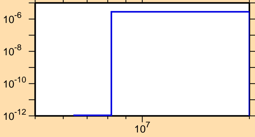
\sigma vs. E for ^{169}\text{Gd}(n,\alpha)
