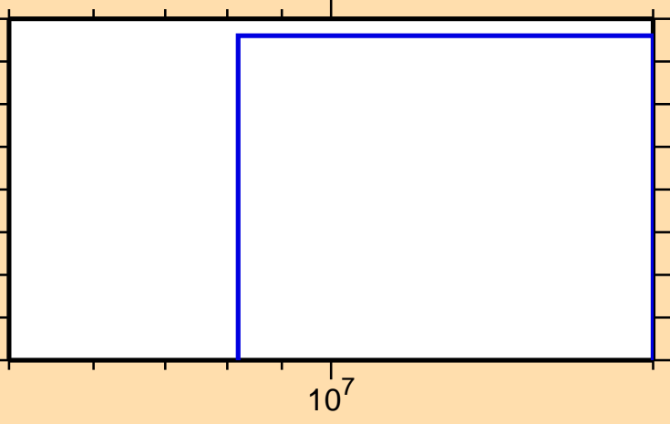
\sigma vs. E for ^{169}\text{Gd}(n,\text{nd})
