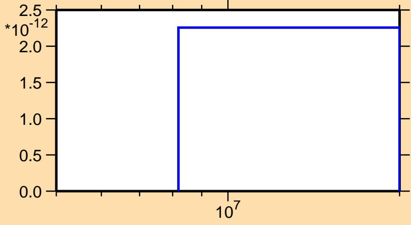
\sigma vs. E for ^{169}\text{Gd}(n,2np)
