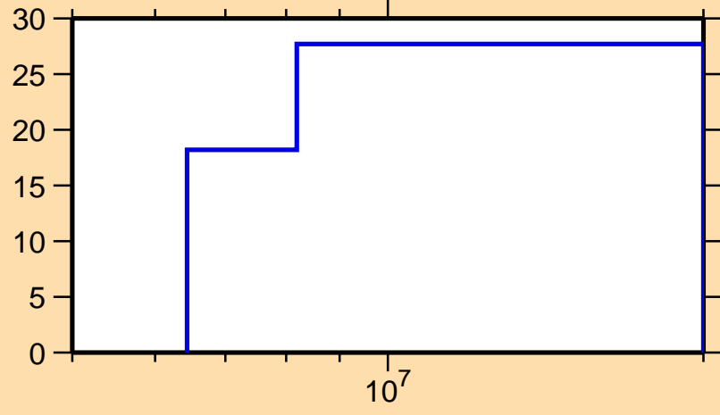
\Delta\sigma/\sigma vs. E for ^{169}\text{Gd}(n,2n)
