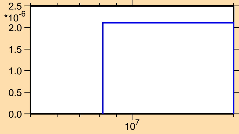
\sigma vs. E for ^{169}\text{Gd}(n,d)
