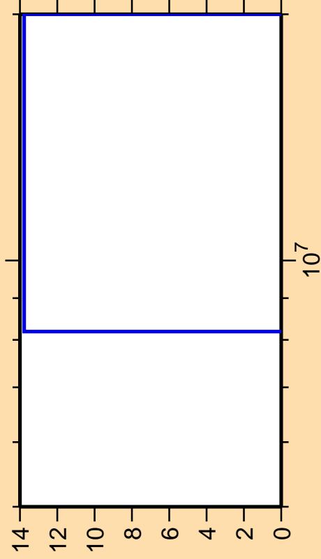
\Delta\sigma/\sigma vs. E for ^{169}\text{Gd}(n,3n)
