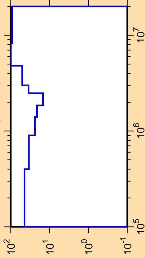
\Delta\sigma/\sigma vs. E for ^{169}\text{Gd}(n,\text{inel.})
