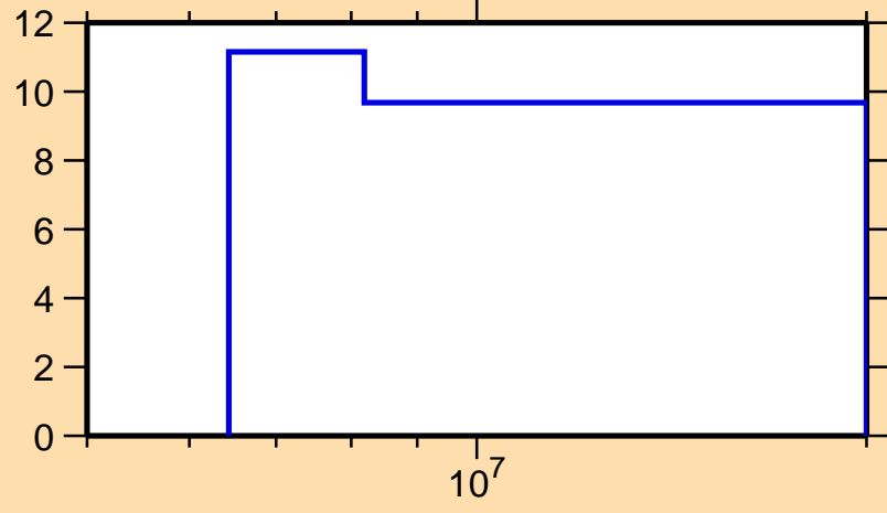
\Delta\sigma/\sigma vs. E for ^{169}\text{Gd}(n,\text{nonel.})
