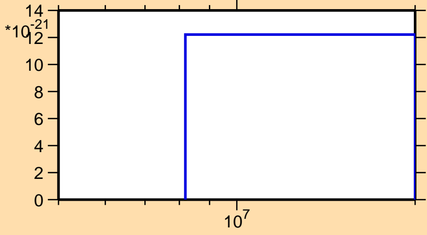
\sigma vs. E for ^{169}\text{Gd}(\text{mt } 11)
