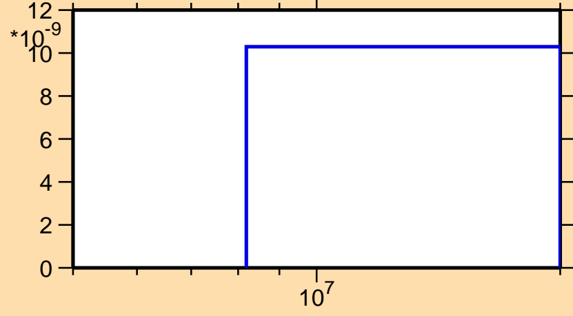
\sigma vs. E for ^{169}\text{Gd}(n,nt)
