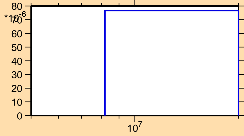
\sigma vs. E for ^{169}\text{Gd}(n,p)
