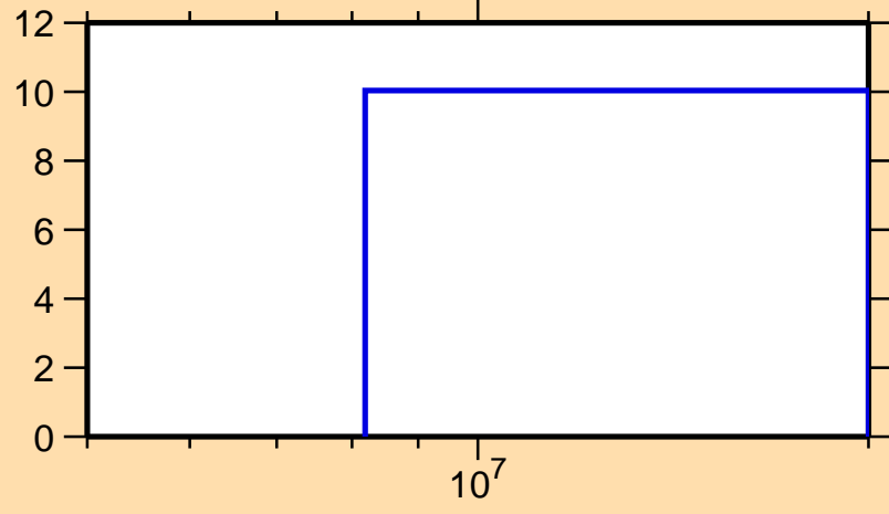
\Delta\sigma/\sigma vs. E for ^{169}\text{Gd}(n,el.)
