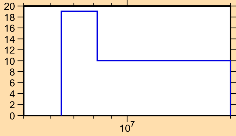
\Delta\sigma/\sigma vs. E for ^{169}\text{Gd}(n,\text{el.})
