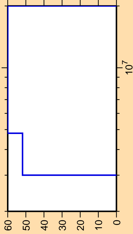
\Delta\sigma/\sigma vs. E for ^{169}\text{Gd}(n,n_{\text{cont}})
