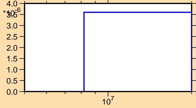
\sigma vs. E for ^{169}\text{Gd}(n,t)
