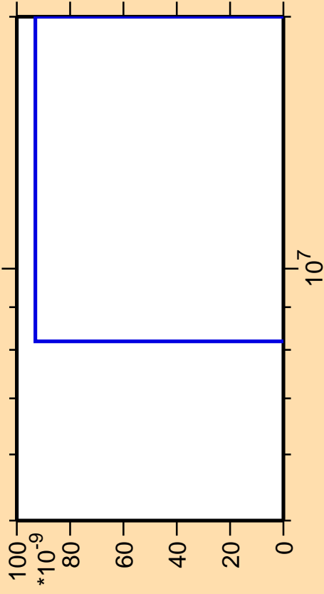
\Delta\sigma/\sigma vs. E for ^{169}\text{Gd}(\text{mt } 11)
