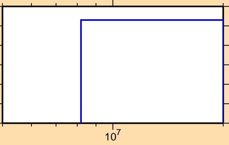
\sigma vs. E for ^{169}\text{Gd}(n,2n\alpha)
