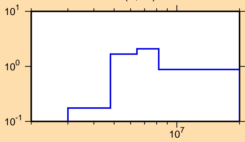
\sigma vs. E for ^{169}\text{Gd}(n,2n)
