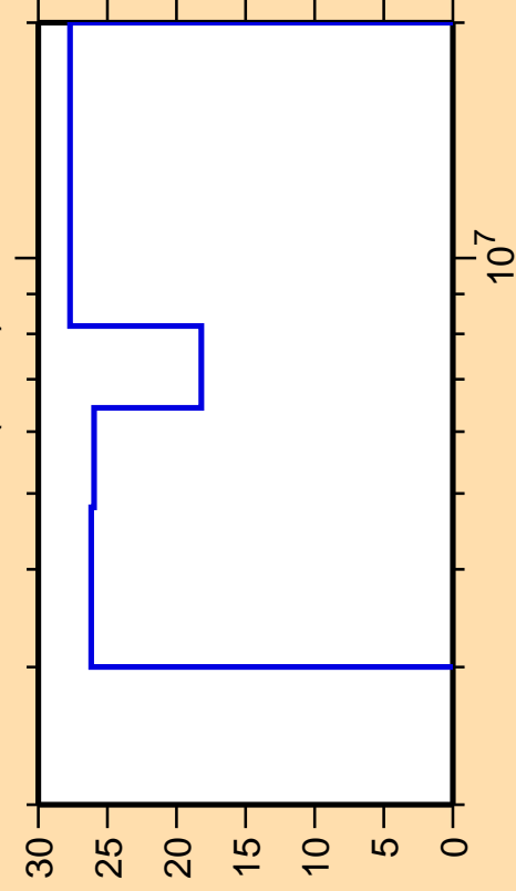
\Delta\sigma/\sigma vs. E for ^{169}\text{Gd}(n,2n)
