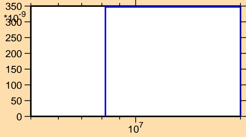
\sigma vs. E for ^{169}\text{Gd}(n,n\alpha)
