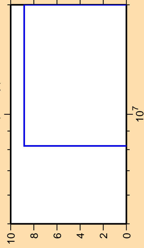
\Delta\sigma/\sigma vs. E for ^{169}\text{Gd}(n,2np)
