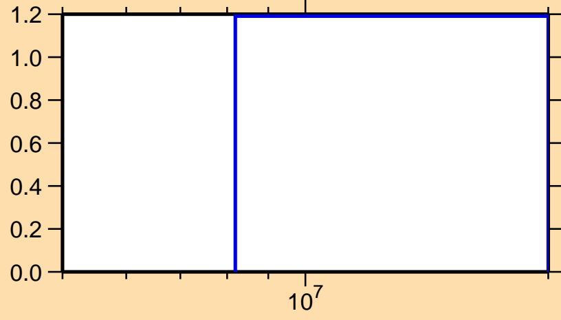
\sigma vs. E for ^{169}\text{Gd}(n,3n)
