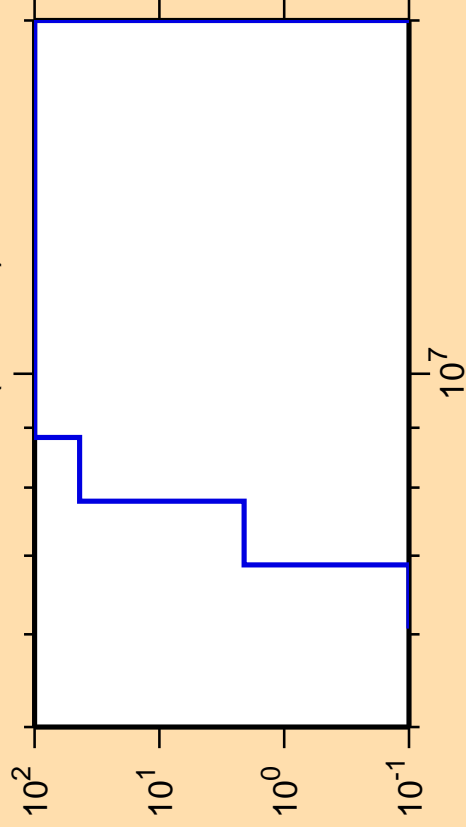
\Delta\sigma/\sigma vs. E for ^{145}\text{Ho}(\text{mt117})
