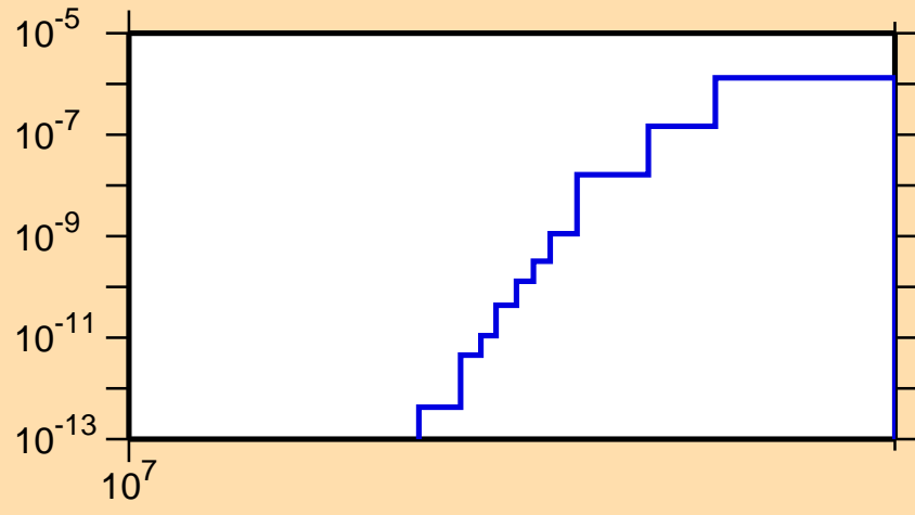
\sigma vs. E for ^{145}\text{Ho}(n,\text{nd})
