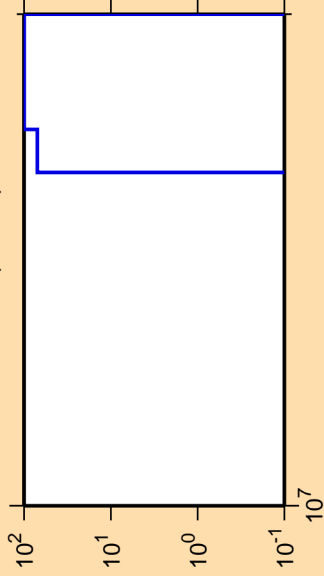
\Delta\sigma/\sigma vs. E for ^{145}\text{Ho} (mt 34)
