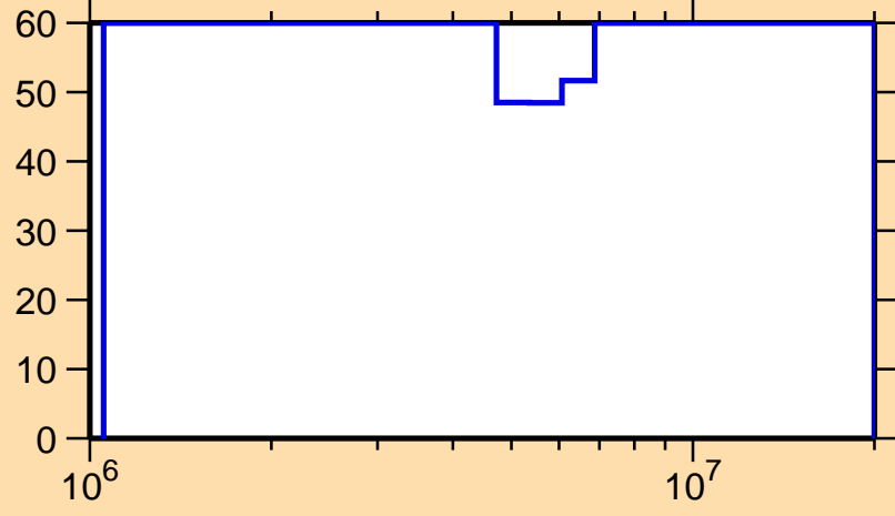
\Delta\sigma/\sigma vs. E for ^{145}\text{Ho}(n,\text{inel.})
