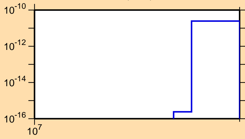
\sigma vs. E for ^{145}\text{Ho}(n,nt)
