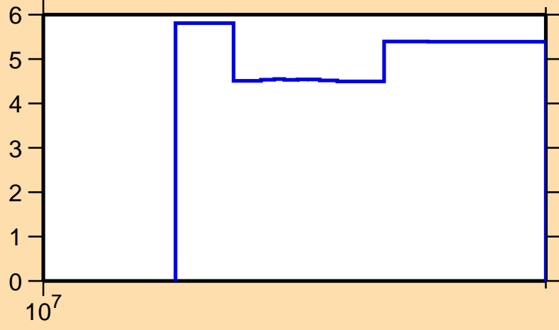
\Delta\sigma/\sigma vs. E for ^{145}\text{Ho}(n,\text{tot.})
