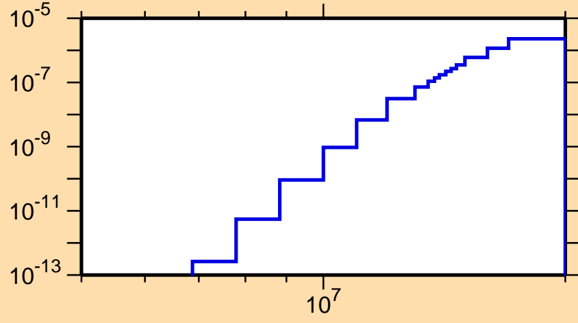
\sigma vs. E for ^{145}\text{Ho}(\text{mt117})
