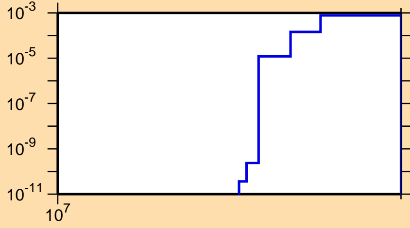
\sigma vs. E for ^{145}\text{Ho}(n,2np)
