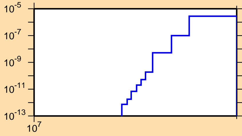
\sigma vs. E for ^{145}\text{Ho}(n,\text{pt})
