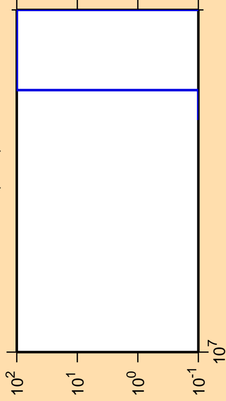
\Delta\sigma/\sigma vs. E for ^{145}\text{Ho}(n,nt)
