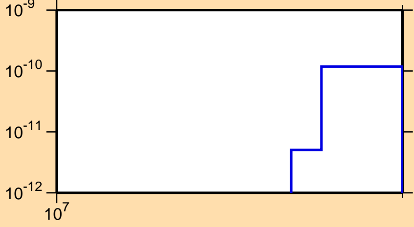
\sigma vs. E for ^{145}\text{Ho}(n,2n\alpha)
