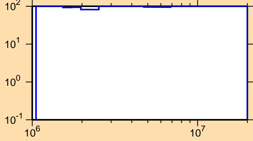
\Delta\sigma/\sigma vs. E for ^{145}\text{Ho}(n,n\text{cont.})
