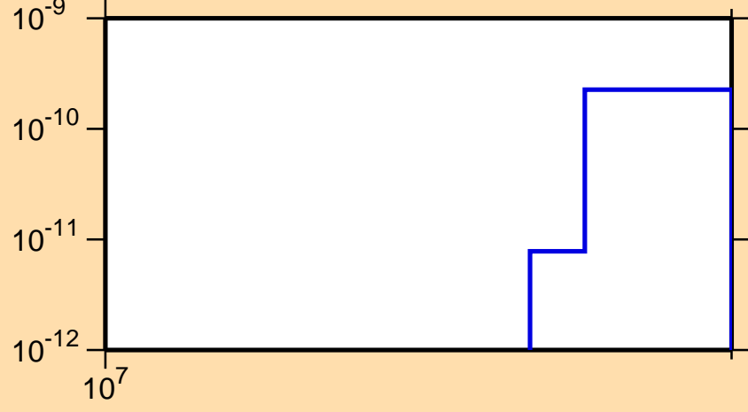
\sigma vs. E for ^{145}\text{Ho} (mt 34)
