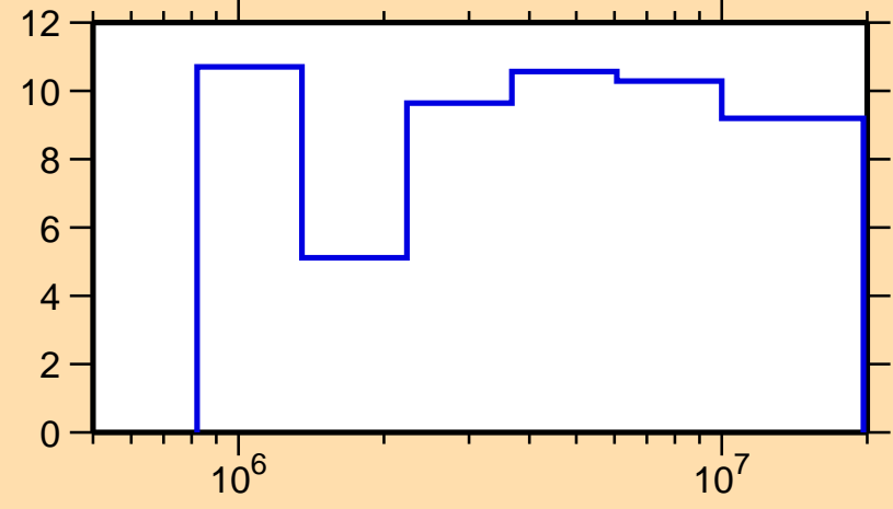
\Delta\sigma/\sigma vs. E for ^{145}\text{Ho}(n,n\text{onel.})
