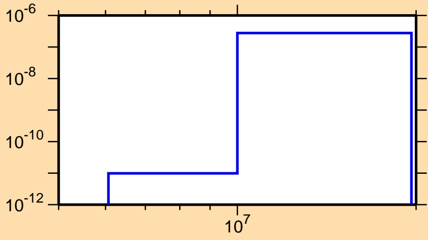
\sigma vs. E for ^{145}\text{Ho}(\text{mt117})
