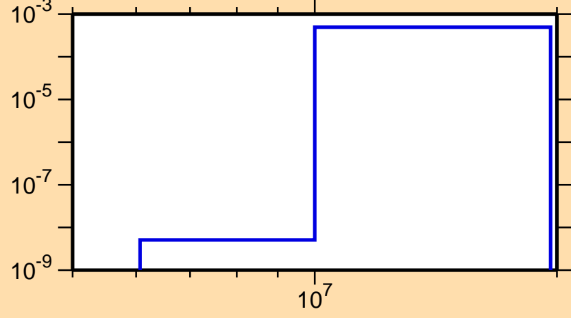
\sigma vs. E for ^{145}\text{Ho}(n,\text{pd})
