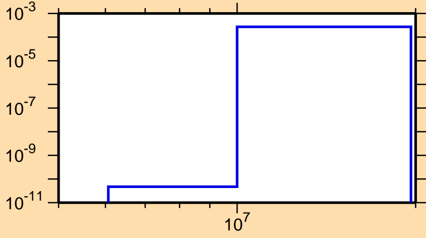
\sigma vs. E for ^{145}\text{Ho}(n,t)
