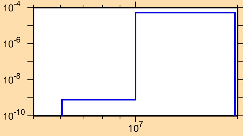
\sigma vs. E for ^{145}\text{Ho} (mt 45)
