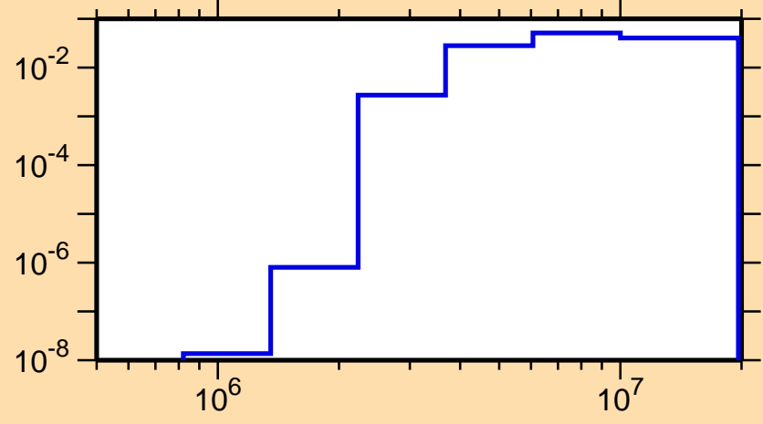
\sigma vs. E for ^{145}\text{Ho}(n,n\text{cont.})
