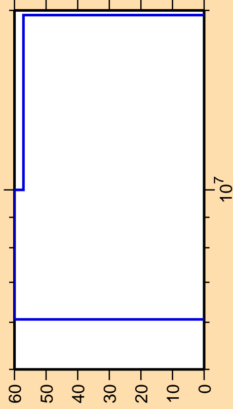
\Delta\sigma/\sigma vs. E for ^{145}\text{Ho} (mt 45)
