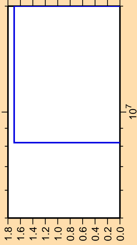
\Delta\sigma/\sigma vs. E for ^{145}\text{Ho}(n,\text{nt})
