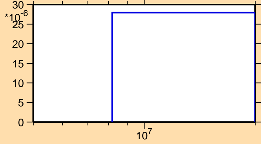
\sigma vs. E for ^{145}\text{Ho}(n,2n)
