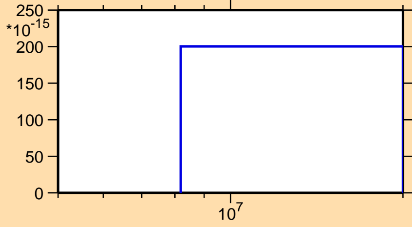
\sigma vs. E for ^{145}\text{Ho}(n,\text{nt})
