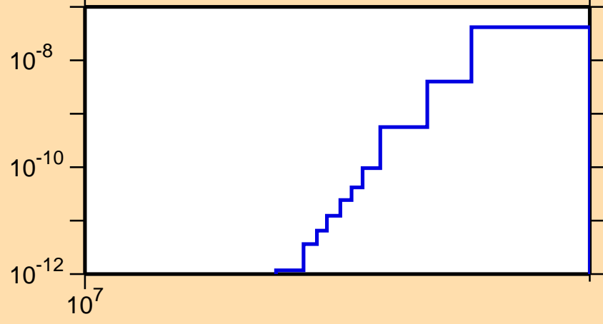
\sigma vs. E for ^{146}\text{Ho} (mt 34)
