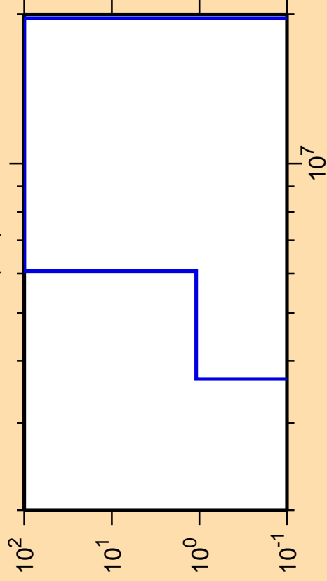
\Delta\sigma/\sigma vs. E for ^{146}\text{Ho}(n,t)
