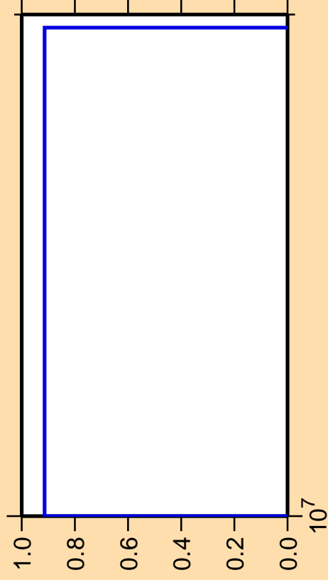
\Delta\sigma/\sigma vs. E for ^{146}\text{Ho}(n,nt)
