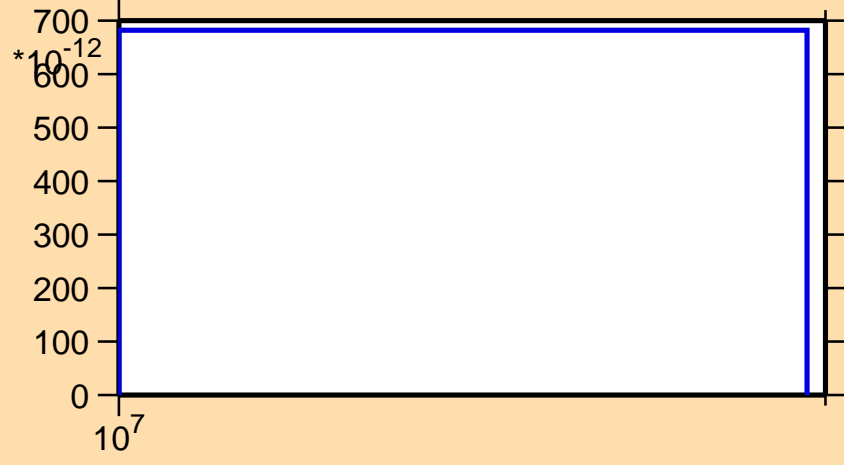
\sigma vs. E for ^{146}\text{Ho} (mt 34)
