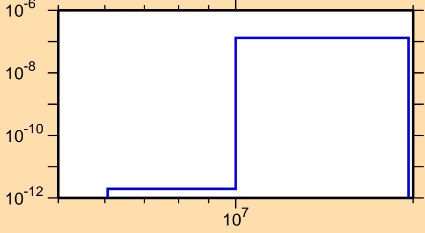
\sigma vs. E for ^{146}\text{Ho}(\text{mt117})
