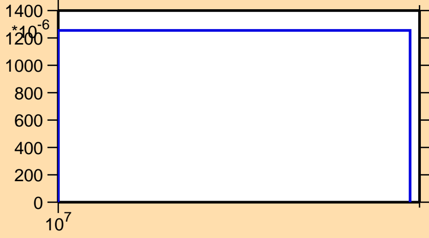
\sigma vs. E for ^{146}\text{Ho}(n,2n)
