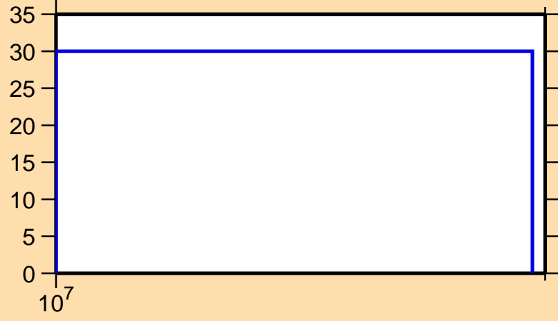
\Delta\sigma/\sigma vs. E for ^{146}\text{Ho}(n,\text{el.})
