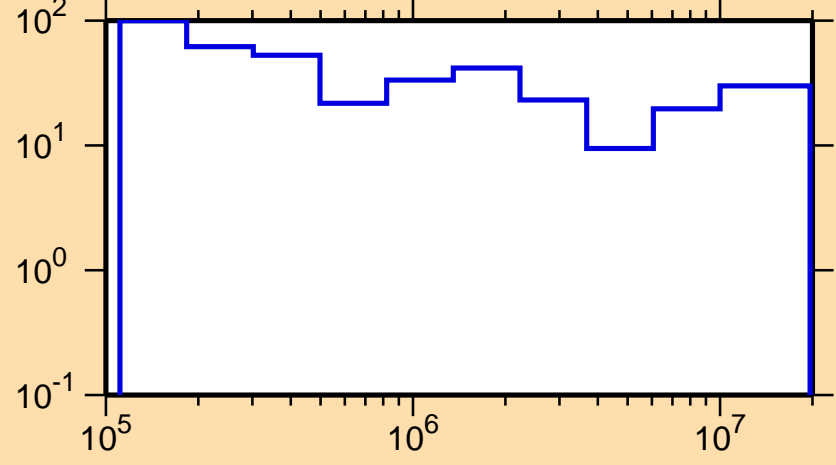
\Delta\sigma/\sigma vs. E for ^{146}\text{Ho}(n,\text{el.})
