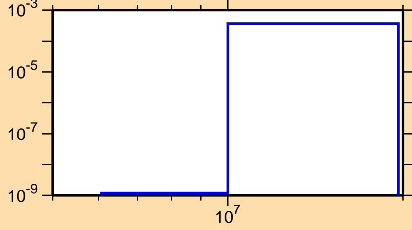
\sigma vs. E for ^{146}\text{Ho}(n,\text{pd})
