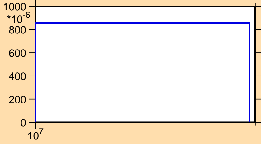
\sigma vs. E for ^{146}\text{Ho}(n,2np)
