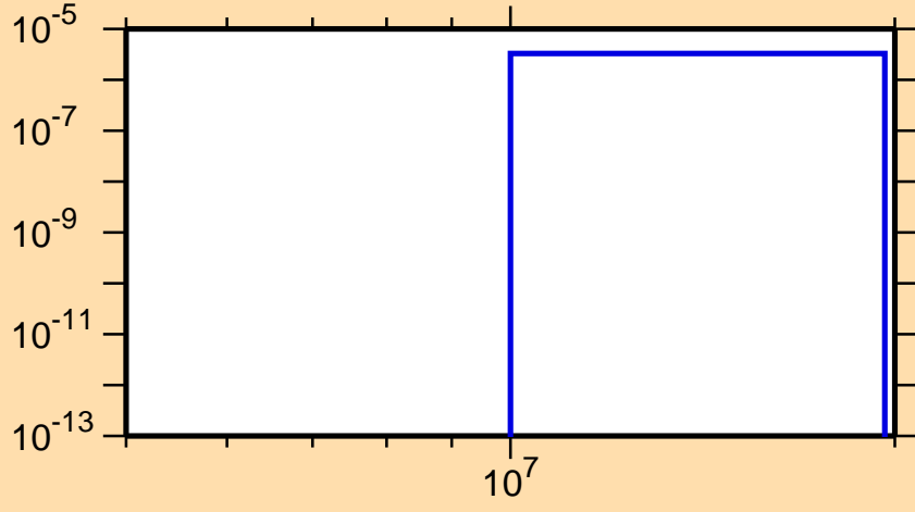
\sigma vs. E for ^{146}\text{Ho}(n,\text{pt})
