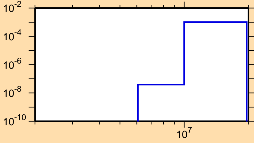
\sigma vs. E for ^{146}\text{Ho}(n,t)
