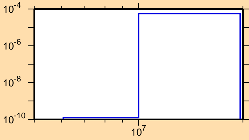
\sigma vs. E for ^{146}\text{Ho} (mt 45)
