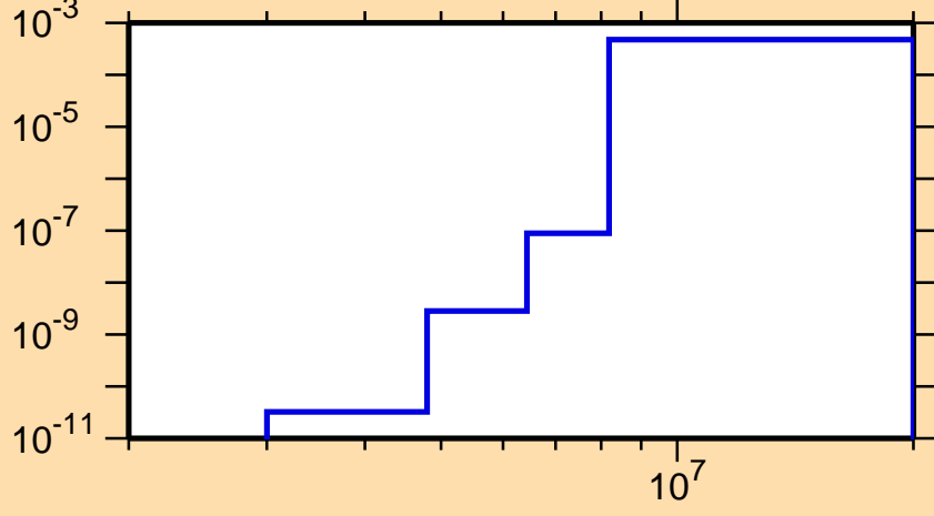
\sigma vs. E for ^{146}\text{Ho}(n,\text{He3})
