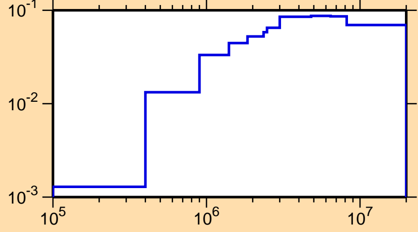
\sigma vs. E for ^{146}\text{Ho}(n,n\text{cont.})
