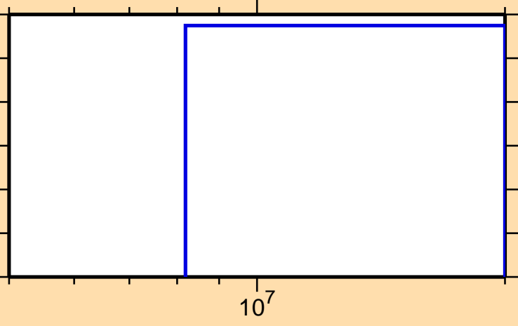
\sigma vs. E for ^{146}\text{Ho}(\text{mt } 34)
