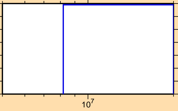
\sigma vs. E for ^{146}\text{Ho}(n,2np)
