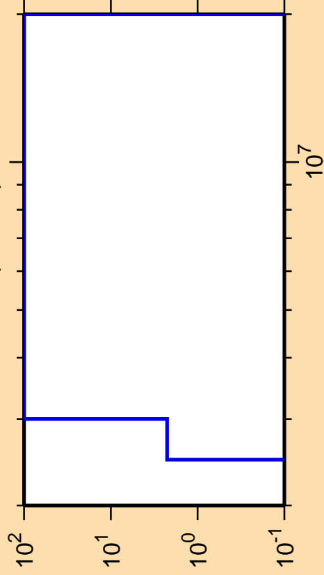
\Delta\sigma/\sigma vs. E for ^{146}\text{Ho}(n,\text{He3})
