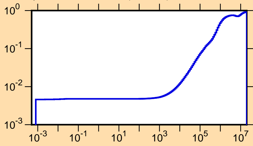
\mu vs. E for ^{147}\text{Ho}(\text{mt251})
