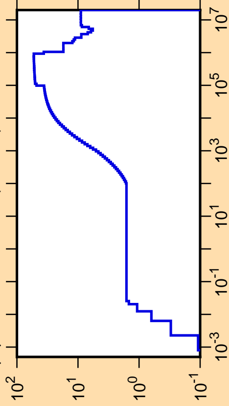
\Delta\mu/\mu vs. E for ^{147}\text{Ho}(\text{mt251})
