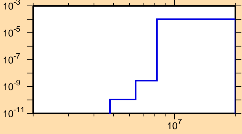
\sigma vs. E for ^{147}\text{Ho}(n,\text{He3})
