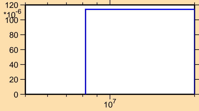
\sigma vs. E for ^{147}\text{Ho}(n,t)
