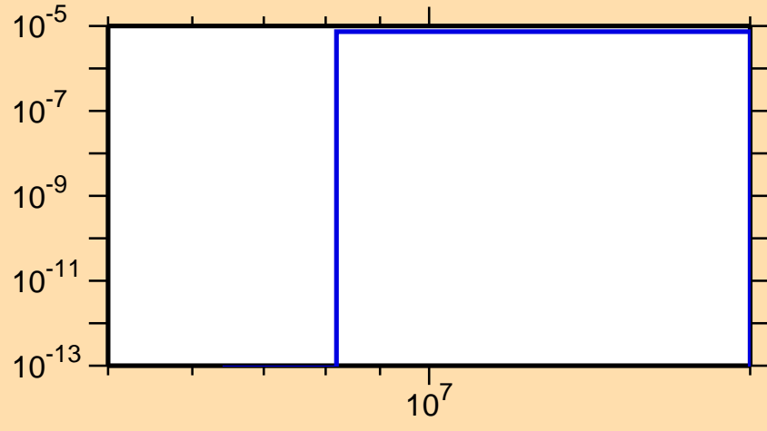
\sigma vs. E for ^{147}\text{Ho}(\text{mt } 45)
