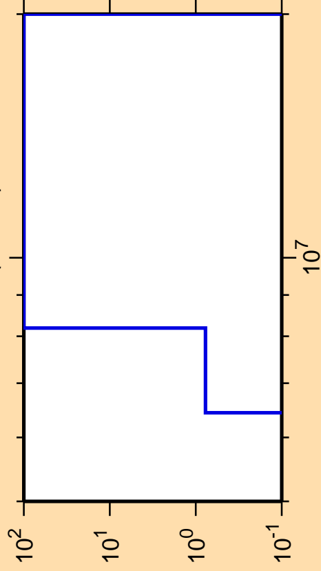
\Delta\sigma/\sigma vs. E for ^{147}\text{Ho}(\text{mt } 45)
