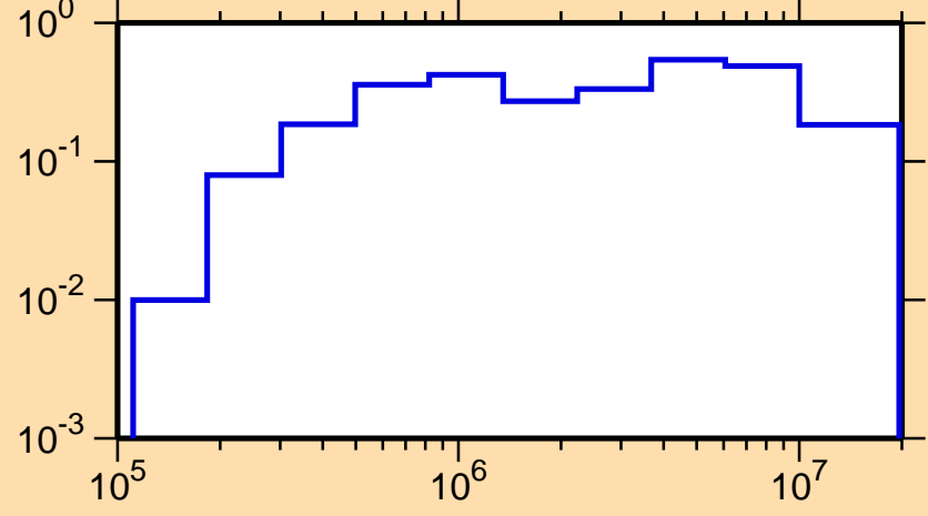
\sigma vs. E for ^{148}\text{Ho}(n,\text{inel.})
