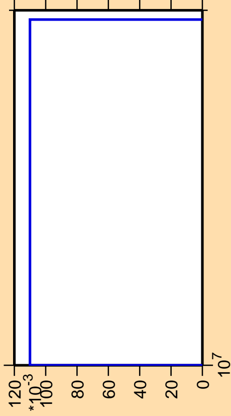
\Delta\sigma/\sigma vs. E for ^{148}\text{Ho}(n,\text{nt})
