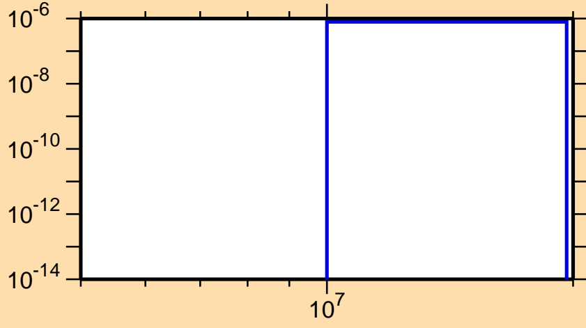
\sigma vs. E for ^{148}\text{Ho}(n,\text{pt})
