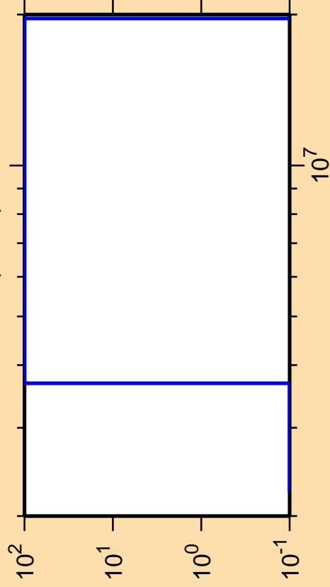
\Delta\sigma/\sigma vs. E for ^{148}\text{Ho}(n,n\alpha)
