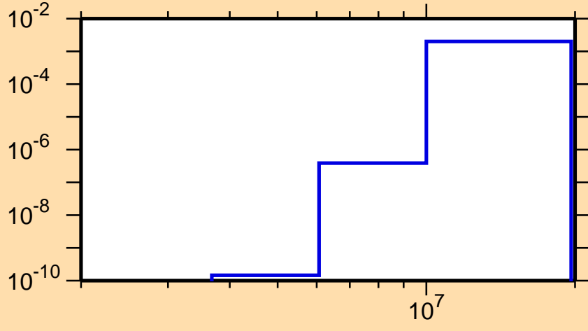
\sigma vs. E for ^{148}\text{Ho}(n,n\alpha)
