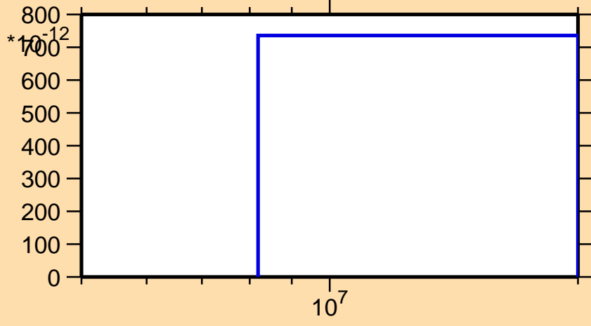
\sigma vs. E for ^{148}\text{Ho}(\text{mt } 34)
