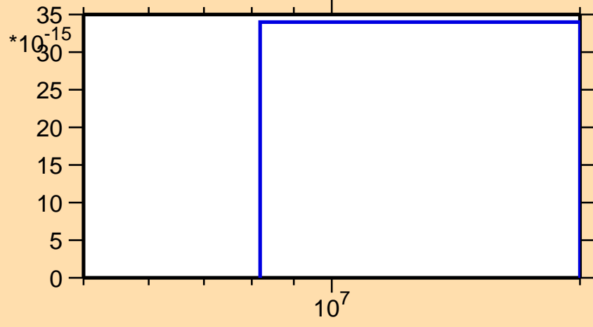
\sigma vs. E for ^{148}\text{Ho}(n,\text{nt})
