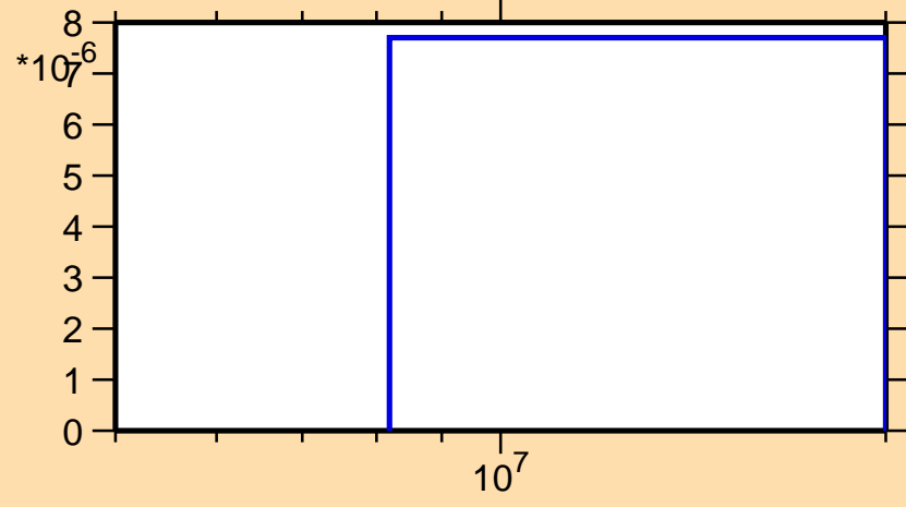
\sigma vs. E for ^{148}\text{Ho}(\text{mt } 45)
