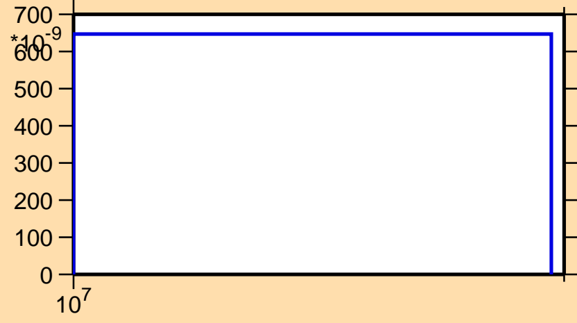
\sigma vs. E for ^{148}\text{Ho}(n,\text{pt})
