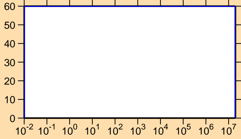
\Delta\sigma/\sigma vs. E for ^{148}\text{Ho}(n,n\text{cont.})
