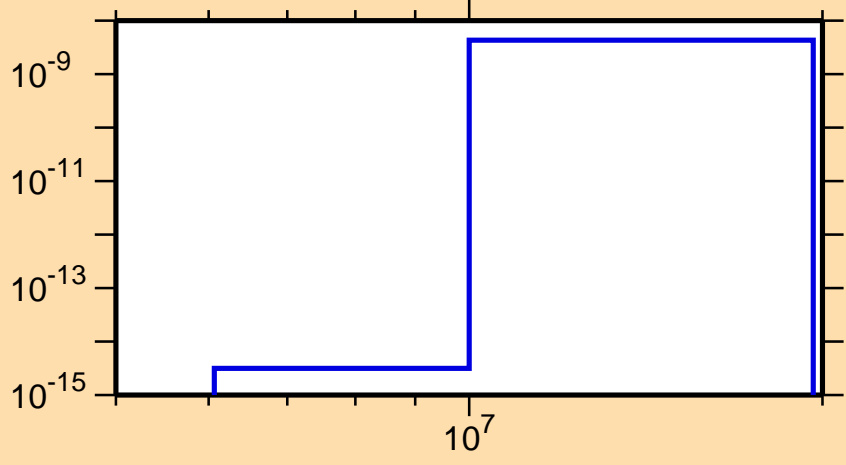
\sigma vs. E for ^{148}\text{Ho}(\text{mt117})
