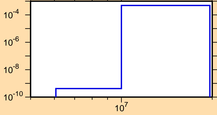
\sigma vs. E for ^{148}\text{Ho}(n,t)
