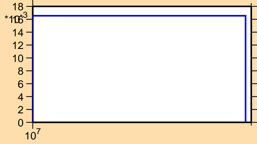
\sigma vs. E for ^{148}\text{Ho}(n,2n)
