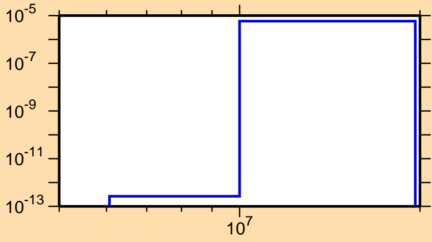
\sigma vs. E for ^{148}\text{Ho}(\text{mt } 45)
