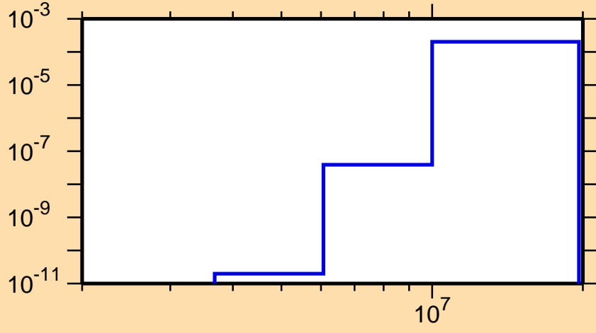
\sigma vs. E for ^{148}\text{Ho}(n,\text{He3})
