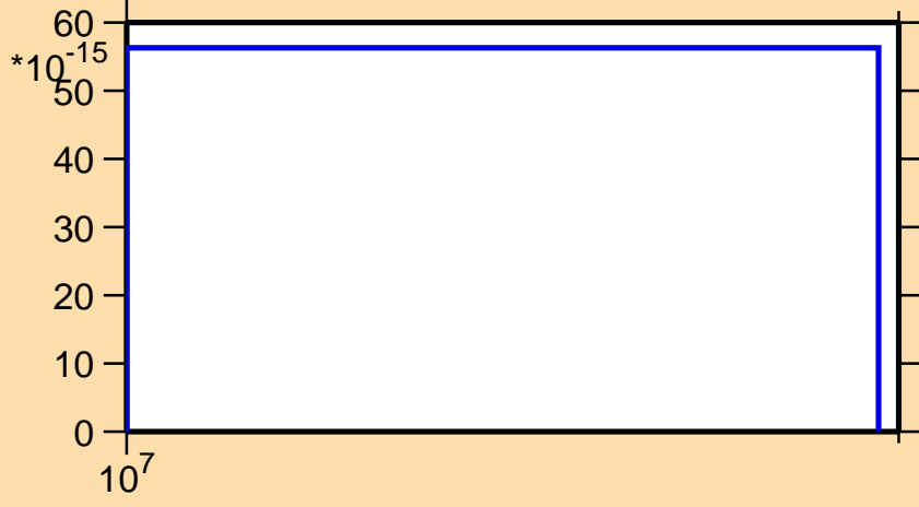
\sigma vs. E for ^{148}\text{Ho}(n,nt)
