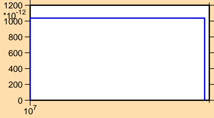
\sigma vs. E for ^{148}\text{Ho} (mt 34)
