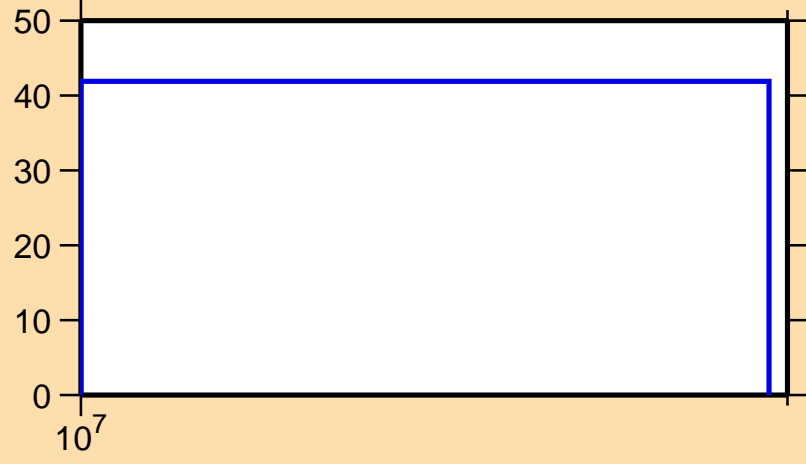
\Delta\sigma/\sigma vs. E for ^{148}\text{Ho}(n,\text{el.})
