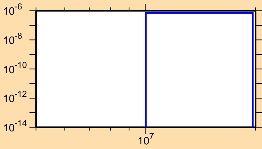
\sigma vs. E for ^{148}\text{Ho}(n,\text{nd})
