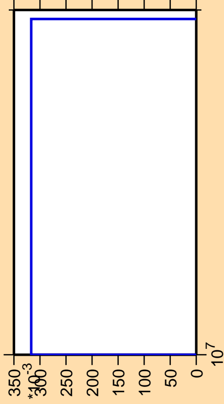
\Delta\sigma/\sigma vs. E for ^{148}\text{Ho}(n,nt)
