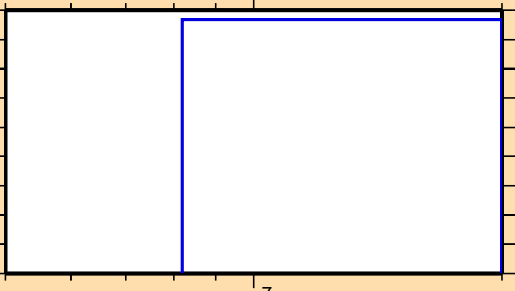
\sigma vs. E for ^{148}\text{Ho}(n,2np)
