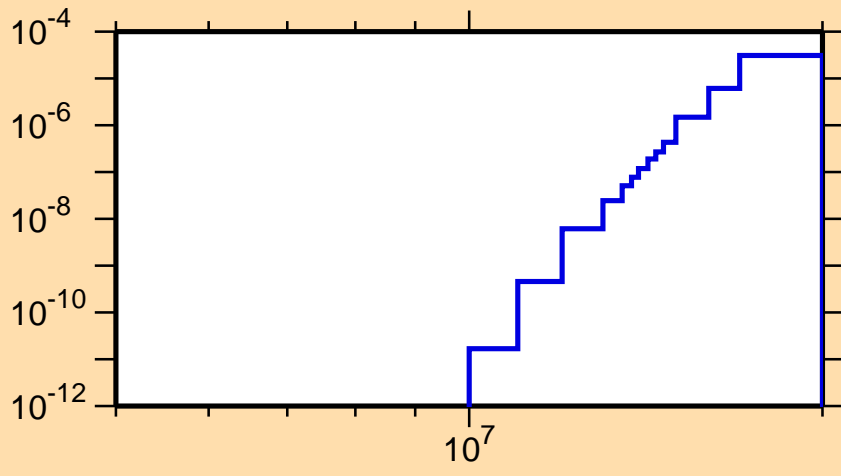
\sigma vs. E for ^{149}\text{Ho}(\text{mt } 45)
