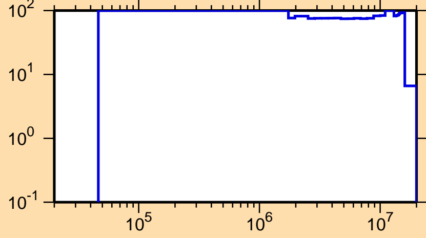
\Delta\sigma/\sigma vs. E for ^{149}\text{Ho}(n,n_1)
