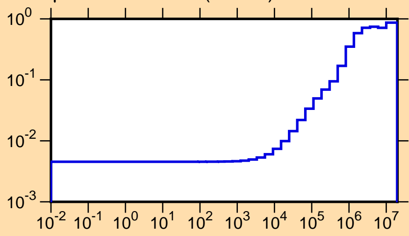
\mu vs. E for ^{149}\text{Ho}(\text{mt251})
