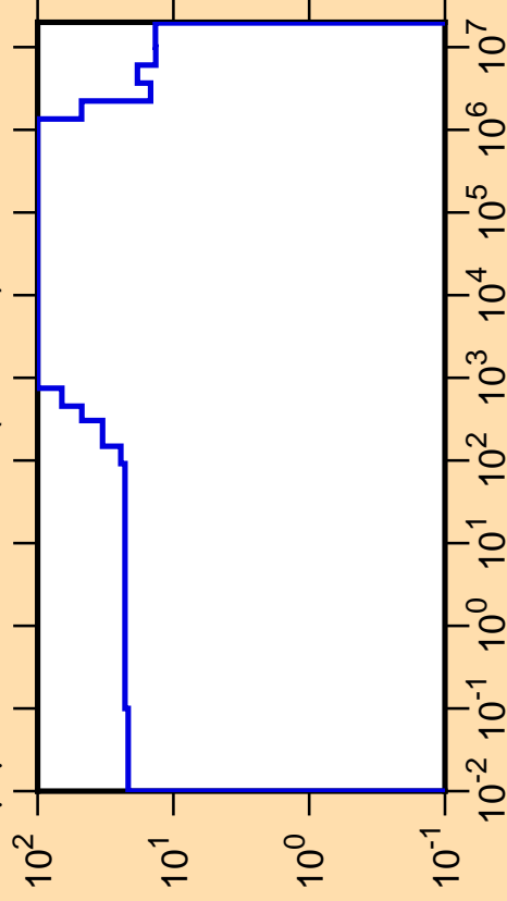
\Delta\mu/\mu vs. E for ^{149}\text{Ho}(\text{mt251})
