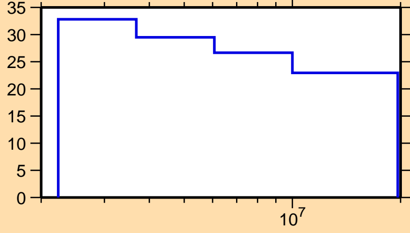
\Delta\sigma/\sigma vs. E for ^{149}\text{Ho}(n,n\text{onel.})
