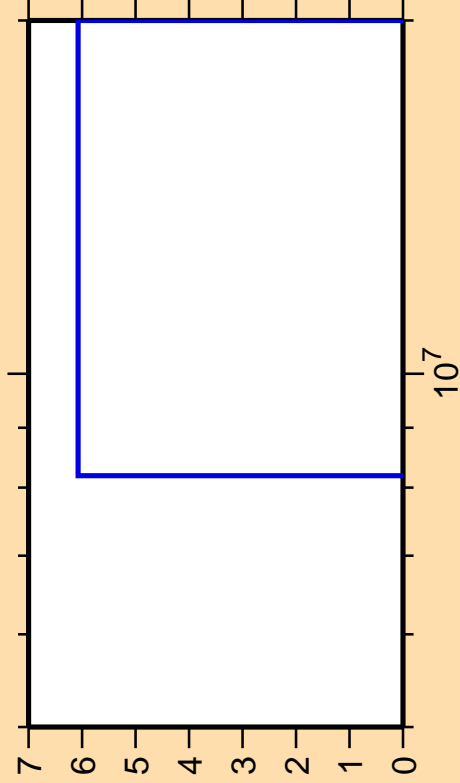
\Delta\sigma/\sigma vs. E for ^{149}\text{Ho}(n,2n\alpha)
