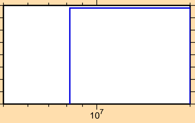
\sigma vs. E for ^{149}\text{Ho}(n,\text{nd})
