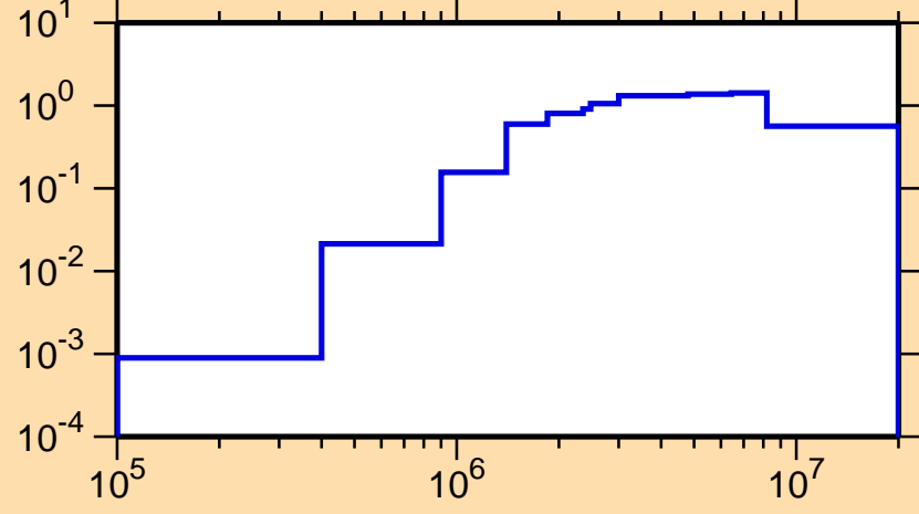
\sigma vs. E for ^{149}\text{Ho}(n,\text{inel.})
