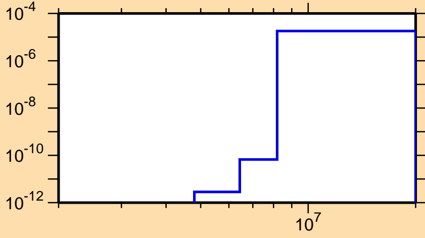
\sigma vs. E for ^{149}\text{Ho}(n,\text{He3})
