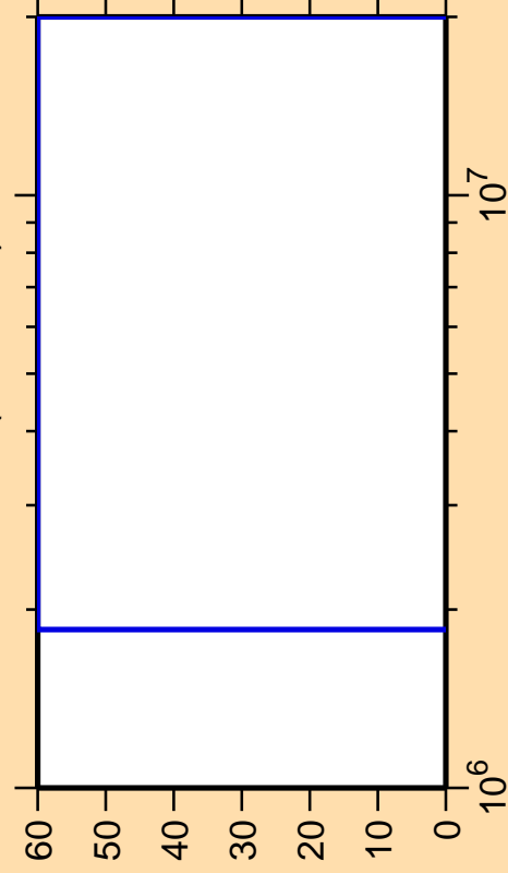
\Delta\sigma/\sigma vs. E for ^{149}\text{Ho}(n,\text{ncont.})
