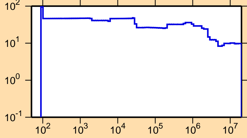
\Delta\sigma/\sigma vs. E for ^{149}\text{Ho}(n,\text{nonel.})
