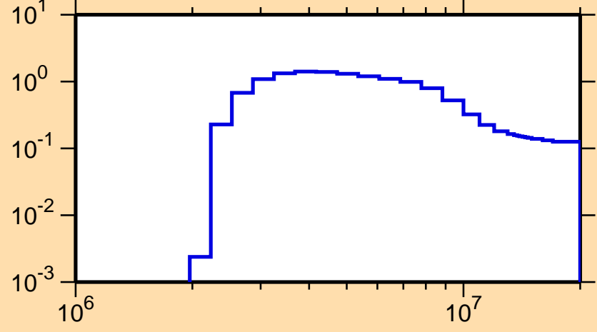
\sigma vs. E for ^{149}\text{Ho}(n,n\text{cont.})
