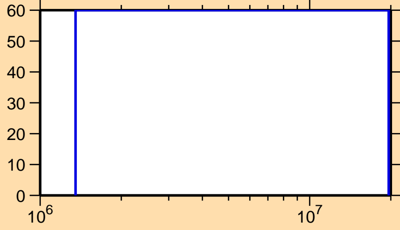
\Delta\sigma/\sigma vs. E for ^{149}\text{Ho}(n,n\text{cont.})
