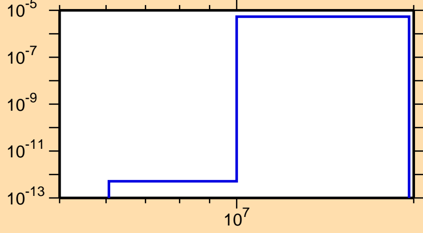
\sigma vs. E for ^{149}\text{Ho}(\text{mt } 45)
