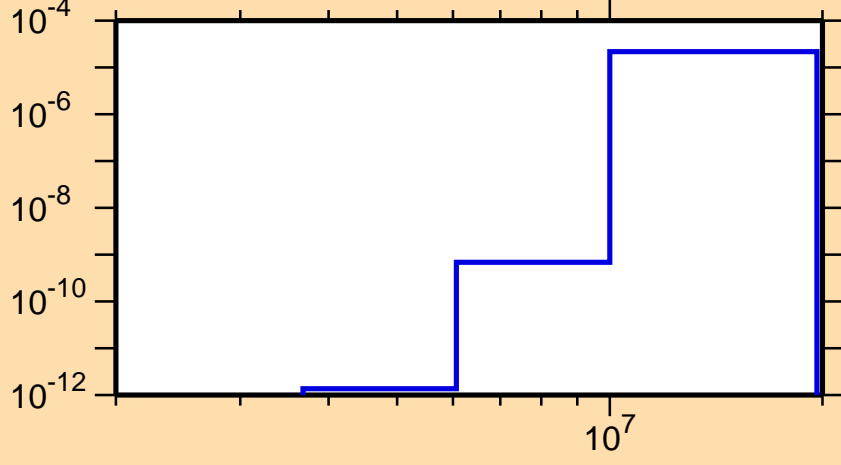
\sigma vs. E for ^{149}\text{Ho}(n,\text{He3})
