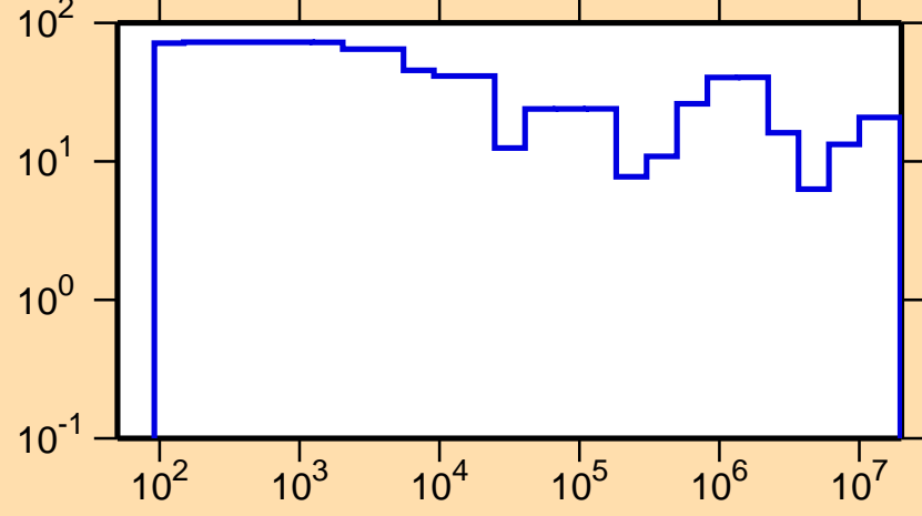
\Delta\sigma/\sigma vs. E for ^{149}\text{Ho}(n,\text{tot.})
