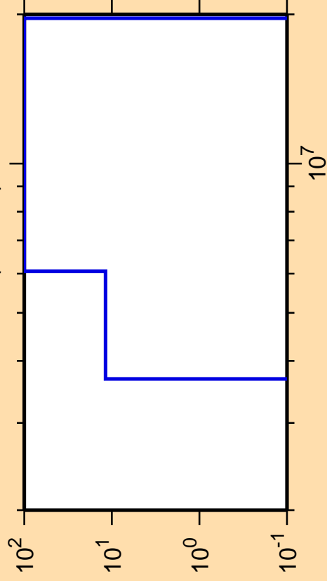
\Delta\sigma/\sigma vs. E for ^{149}\text{Ho}(n,\text{He3})
