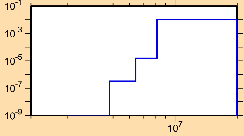
\sigma vs. E for ^{149}\text{Ho}(n,n\alpha)
