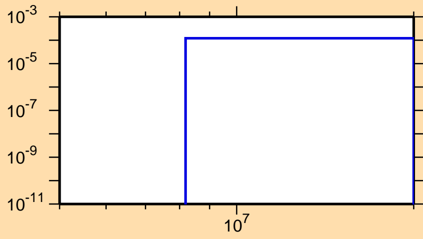
\sigma vs. E for ^{149}\text{Ho}(n,t)
