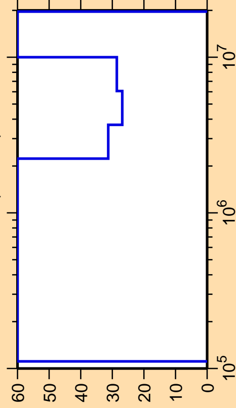
\Delta\sigma/\sigma vs. E for ^{150}\text{Ho}(n,\text{inel.})
