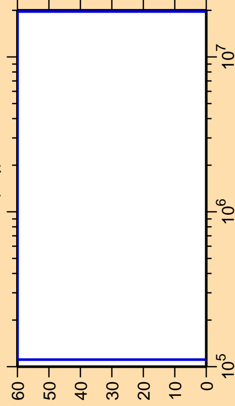
\Delta\sigma/\sigma vs. E for ^{150}\text{Ho}(n,\gamma)
