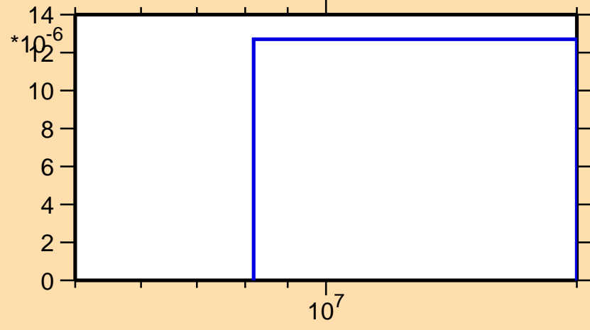
\sigma vs. E for ^{150}\text{Ho}(n,\text{nd})
