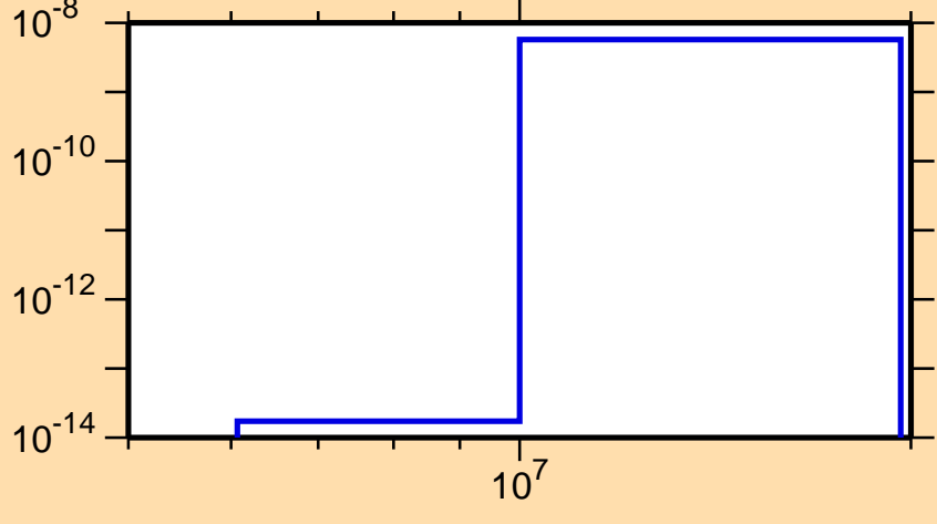
\sigma vs. E for ^{150}\text{Ho}(\text{mt117})
