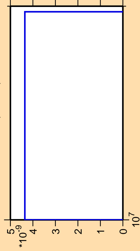
\Delta\sigma/\sigma vs. E for ^{150}\text{Ho} (mt 11)
