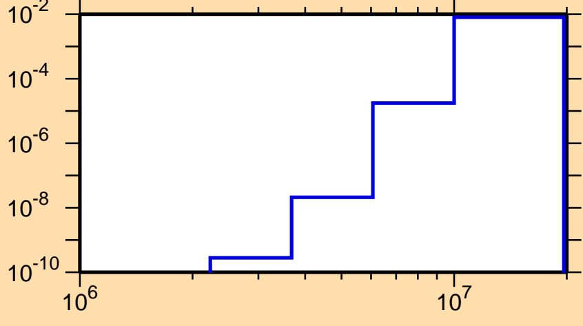
\sigma vs. E for ^{150}\text{Ho}(n,d)
