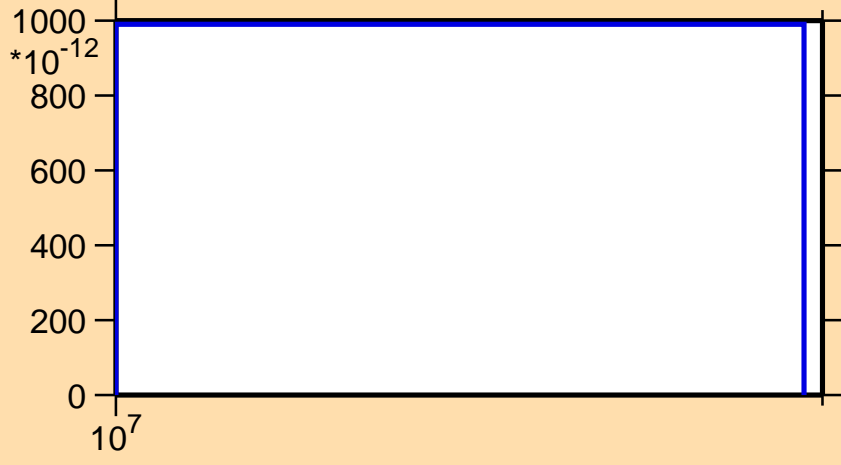
\sigma vs. E for ^{150}\text{Ho} (mt 34)
