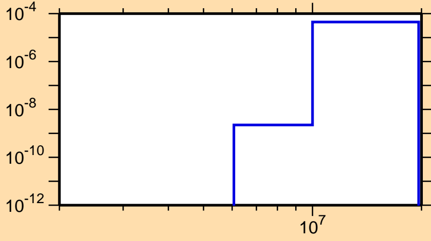
\sigma vs. E for ^{150}\text{Ho}(n,\text{He3})
