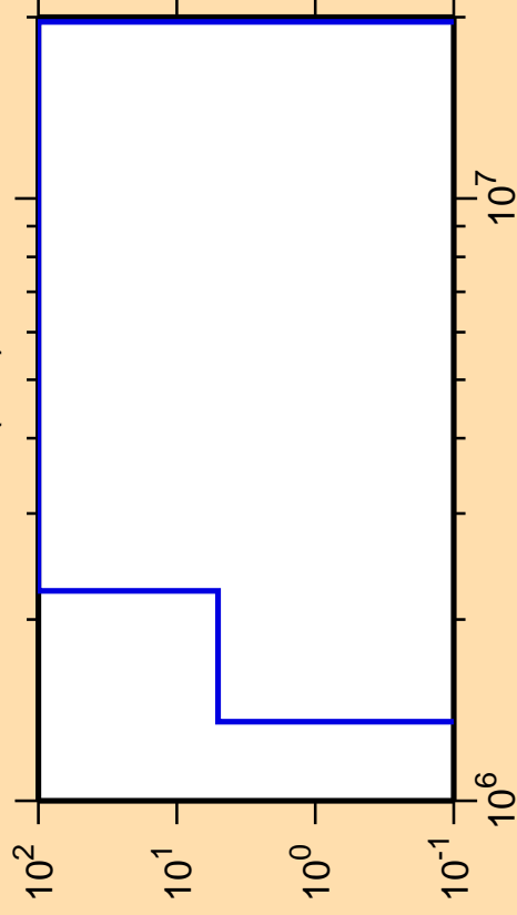
\Delta\sigma/\sigma vs. E for ^{150}\text{Ho}(n,d)
