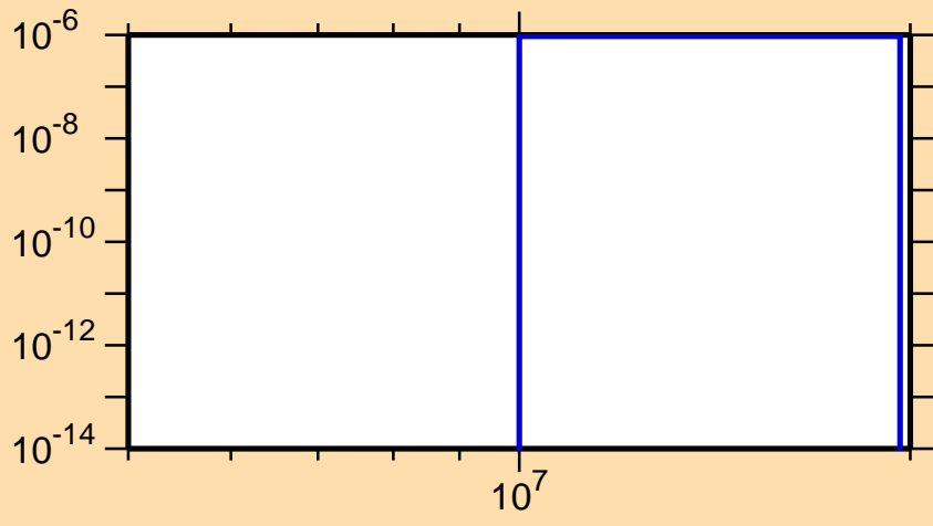
\sigma vs. E for ^{150}\text{Ho}(n,\text{pd})
