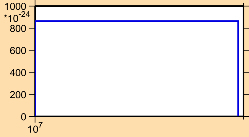
\sigma vs. E for ^{150}\text{Ho} (mt 11)
