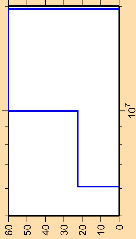
\Delta\sigma/\sigma vs. E for ^{150}\text{Ho} (mt 45)
