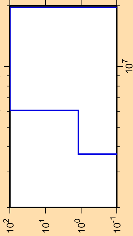
\Delta\sigma/\sigma vs. E for ^{150}\text{Ho}(n,\text{He3})
