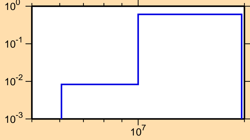
\sigma vs. E for ^{150}\text{Ho}(n,2n)
