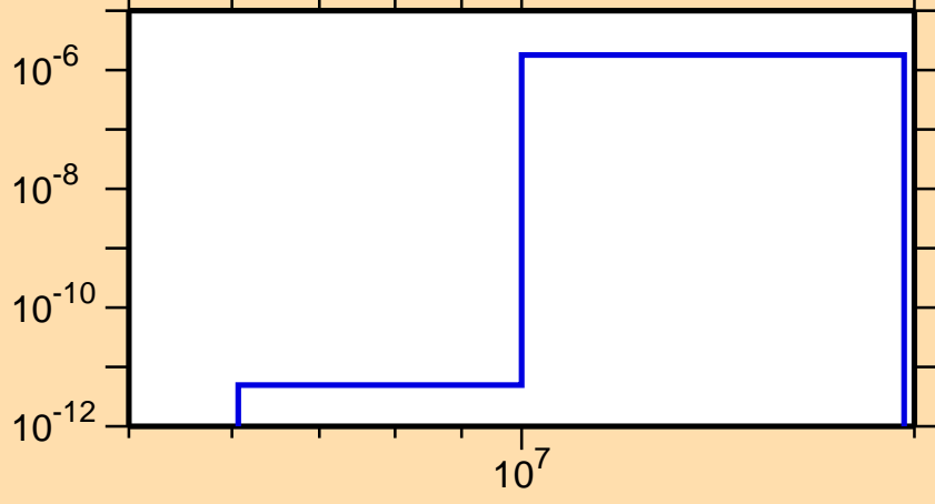
\sigma vs. E for ^{150}\text{Ho} (mt 45)
