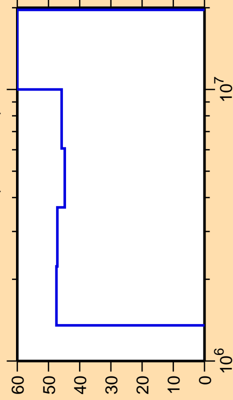
\Delta\sigma/\sigma vs. E for ^{150}\text{Ho}(n,n\text{cont.})
