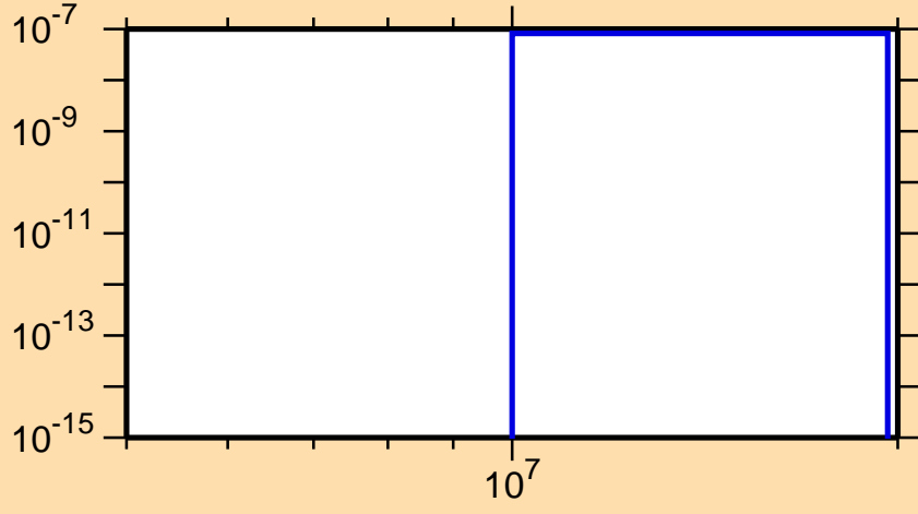
\sigma vs. E for ^{150}\text{Ho}(n,\text{pt})
