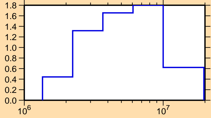
\sigma vs. E for ^{150}\text{Ho}(n,n\text{cont.})
