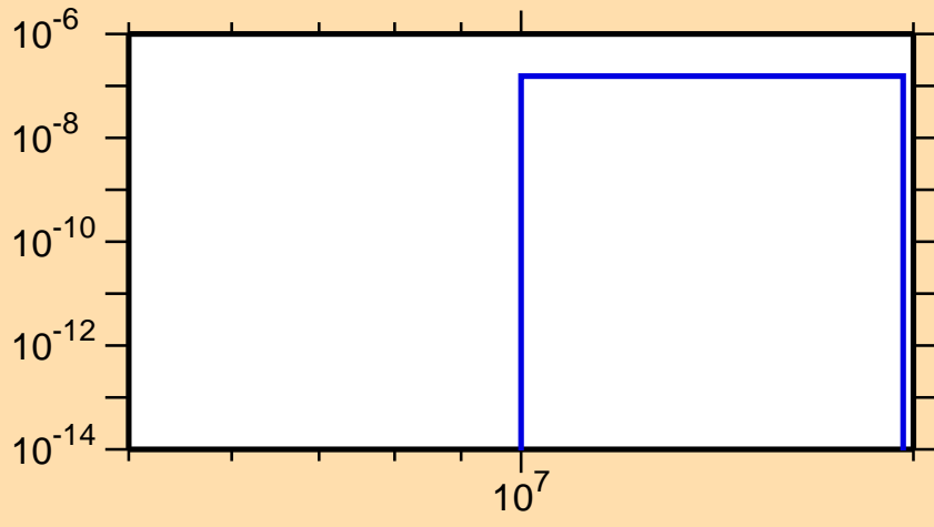
\sigma vs. E for ^{150}\text{Ho}(n,2n\alpha)
