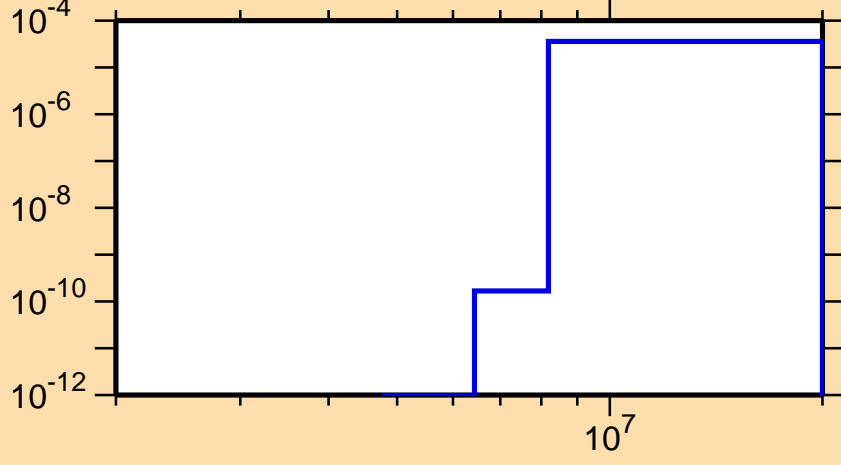
\sigma vs. E for ^{150}\text{Ho}(n,\text{He3})
