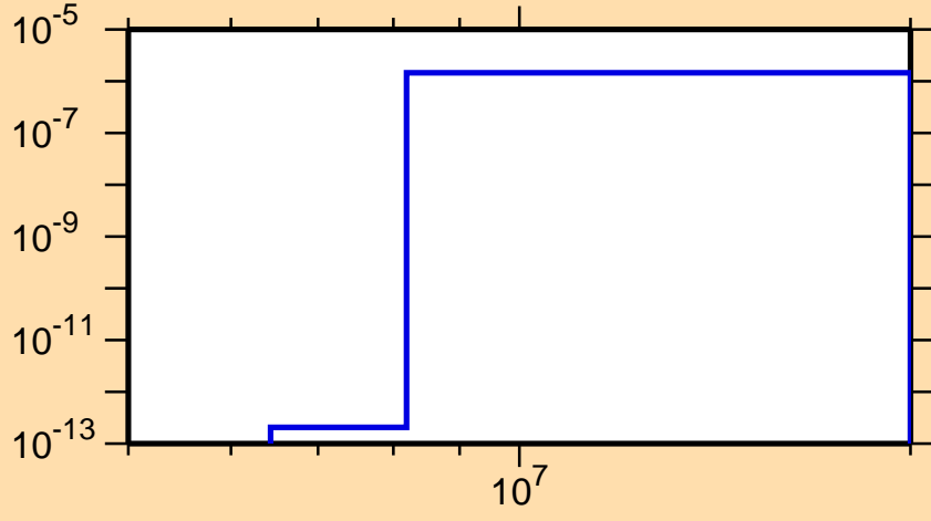
\sigma vs. E for ^{150}\text{Ho} (mt 45)
