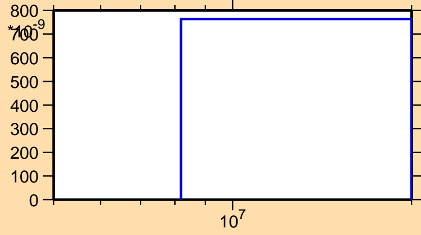
\sigma vs. E for ^{150}\text{Ho}(n,\text{pd})
