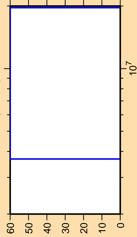
\Delta\sigma/\sigma vs. E for ^{151}\text{Ho} (mt 45)
