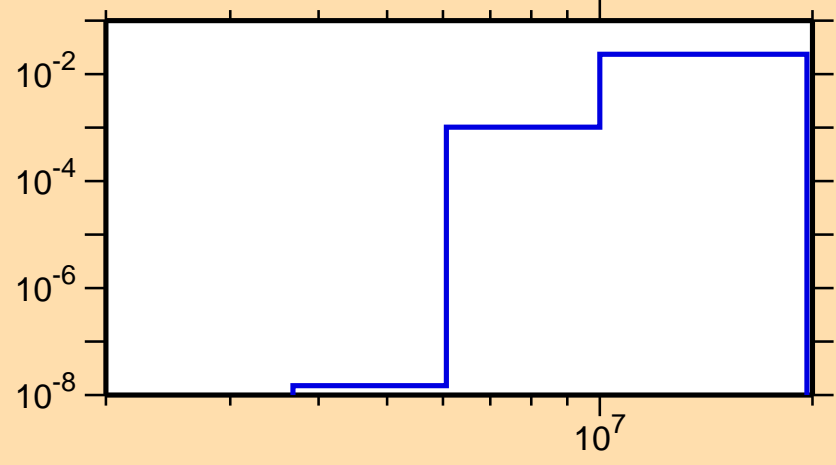
\sigma vs. E for ^{151}\text{Ho} (mt 45)
