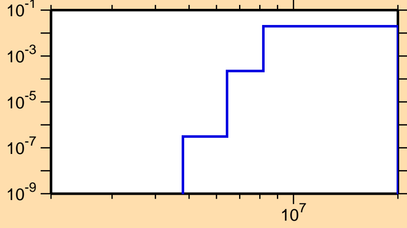
\sigma vs. E for ^{151}\text{Ho} (mt 45)
