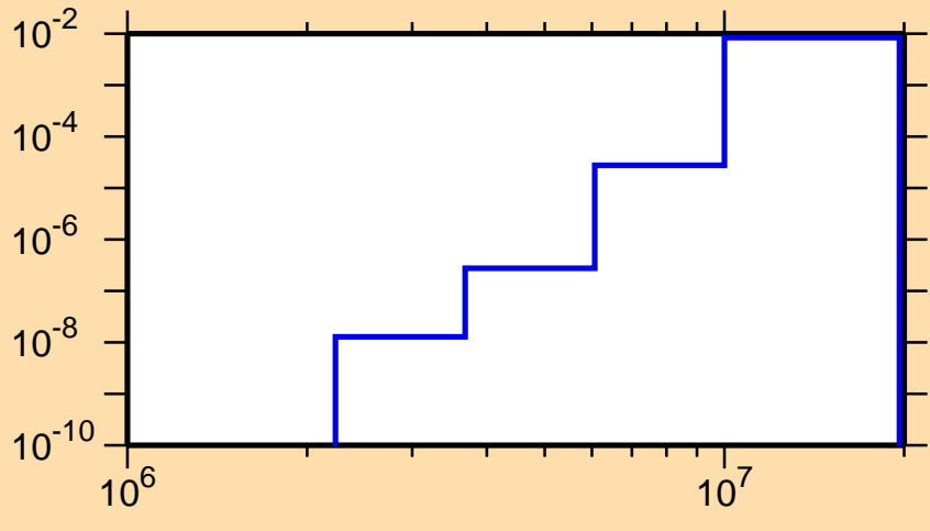
\sigma vs. E for ^{151}\text{Ho}(n,d)
