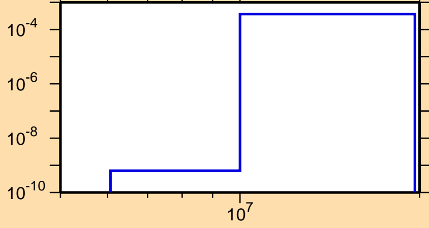
\sigma vs. E for ^{151}\text{Ho}(n,t)
