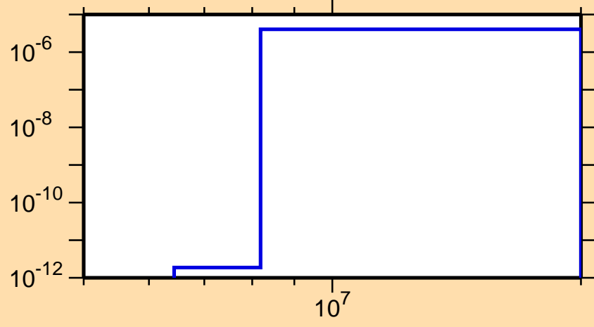
\sigma vs. E for ^{151}\text{Ho}(n,\text{He3})
