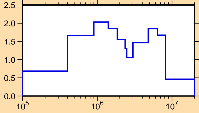
\sigma vs. E for ^{151}\text{Ho}(n,\text{inel.})
