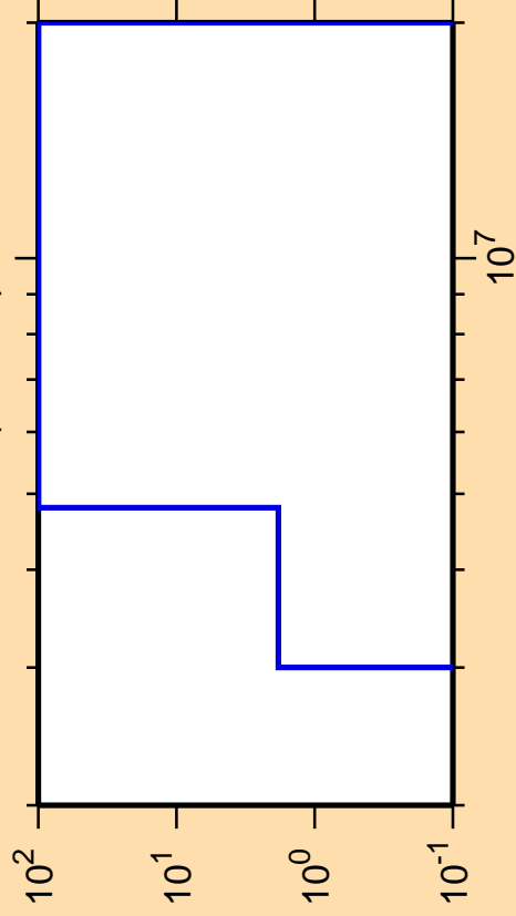
\Delta\sigma/\sigma vs. E for ^{151}\text{Ho}(\text{mt117})
