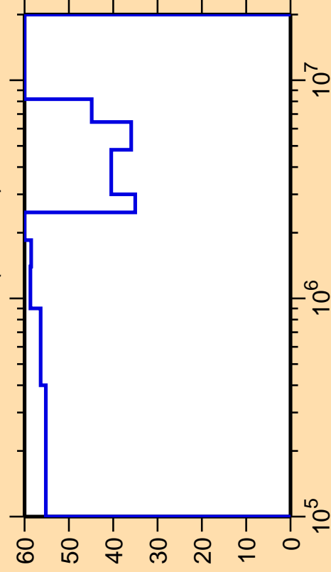
\Delta\sigma/\sigma vs. E for ^{151}\text{Ho}(n,\text{inel.})
