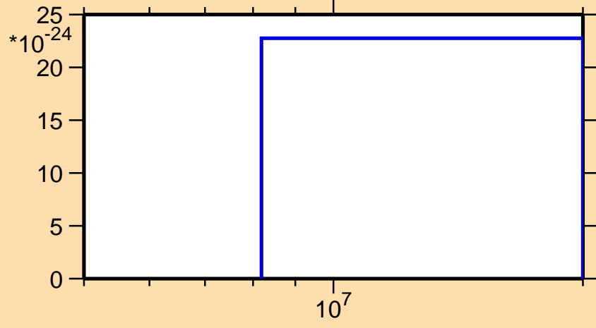
\sigma vs. E for ^{151}\text{Ho} (mt 42)
