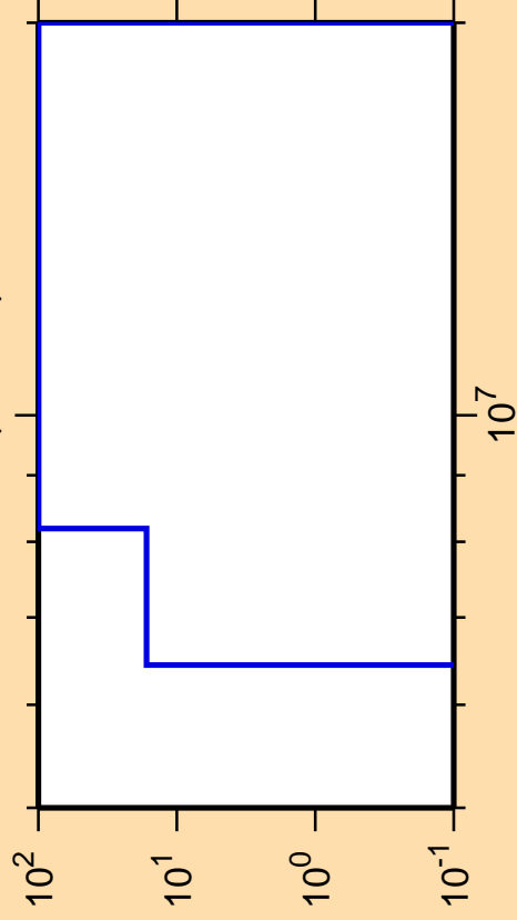
\Delta\sigma/\sigma vs. E for ^{151}\text{Ho}(n,\text{He3})
