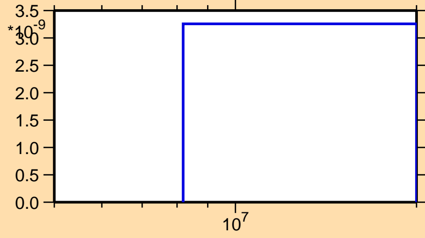
\sigma vs. E for ^{151}\text{Ho}(n,\text{pt})
