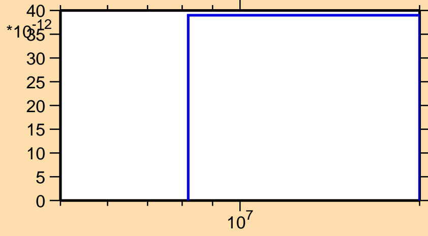
\sigma vs. E for ^{151}\text{Ho} (mt 34)
