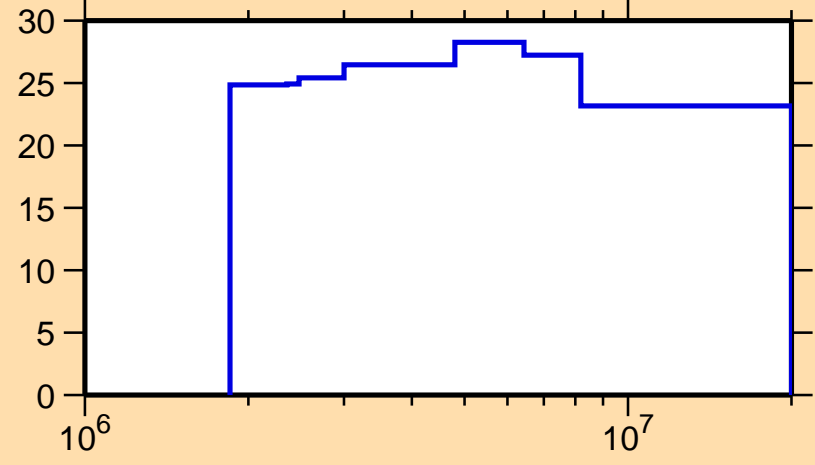
\Delta\sigma/\sigma vs. E for ^{151}\text{Ho}(n,\text{nonel.})
