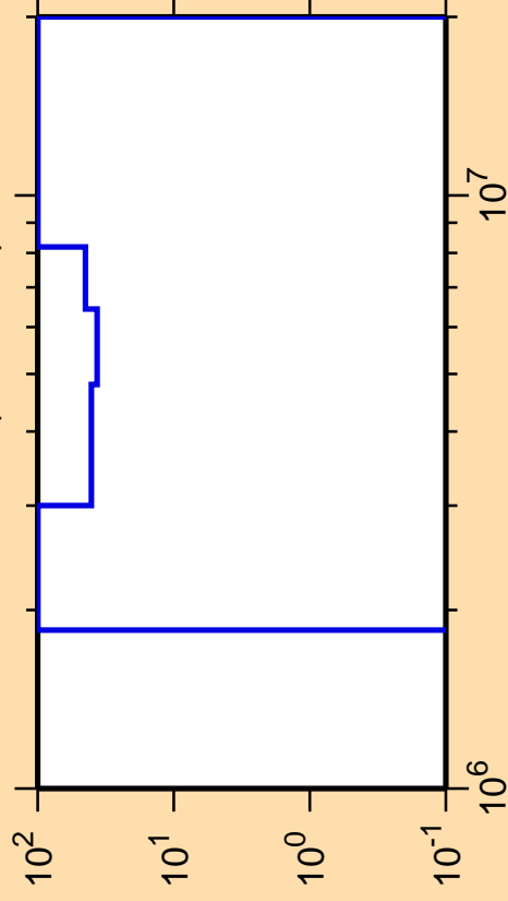
\Delta\sigma/\sigma vs. E for ^{151}\text{Ho}(n,n\text{cont.})
