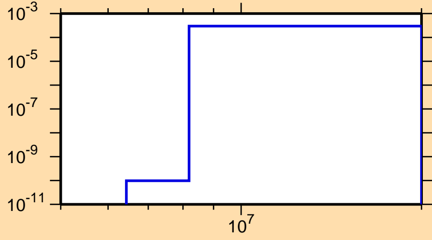
\sigma vs. E for ^{151}\text{Ho}(n,t)
