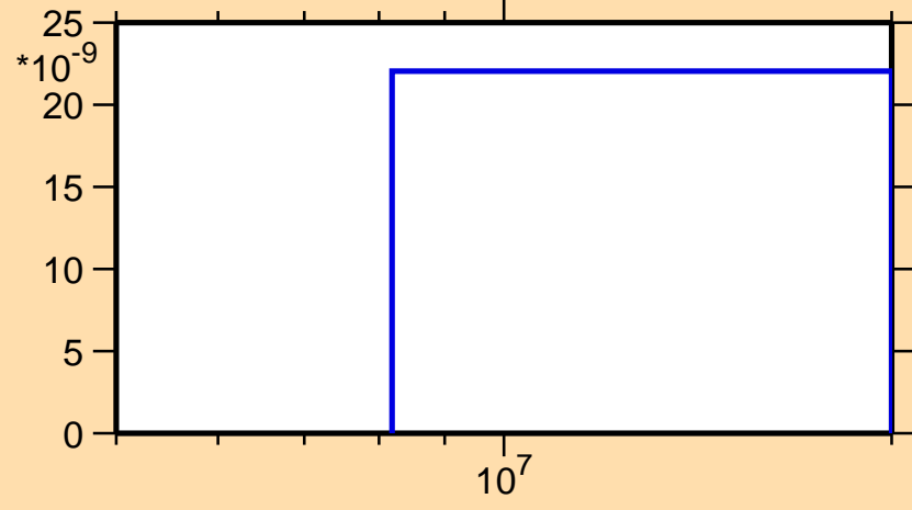
\sigma vs. E for ^{151}\text{Ho}(n,\text{nt})
