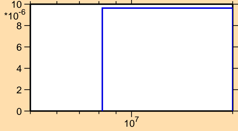
\sigma vs. E for ^{151}\text{Ho}(n,3n)
