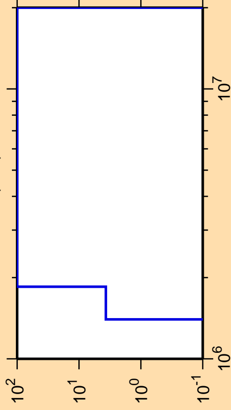
\Delta\sigma/\sigma vs. E for ^{151}\text{Ho}(n,d)
