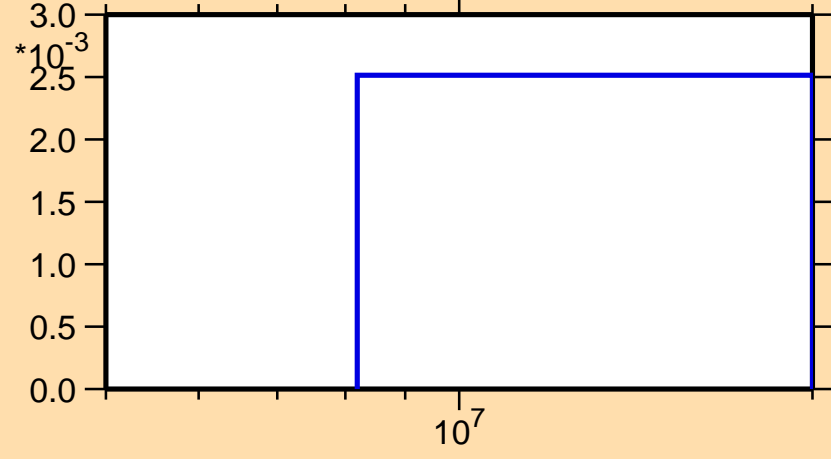
\sigma vs. E for ^{151}\text{Ho}(n,2np)
