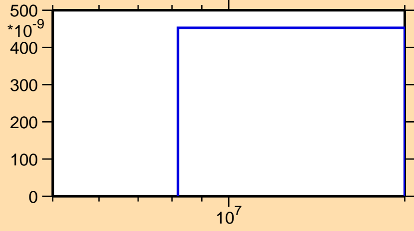
\sigma vs. E for ^{151}\text{Ho}(n,\text{pd})
