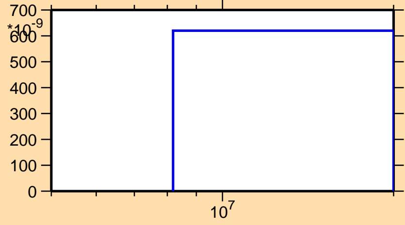
\sigma vs. E for ^{151}\text{Ho}(n,2n\alpha)
