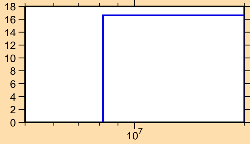
\Delta\sigma/\sigma vs. E for ^{151}\text{Ho}(n,\text{tot.})
