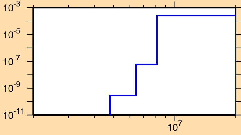
\sigma vs. E for ^{151}\text{Ho}(\text{mt117})
