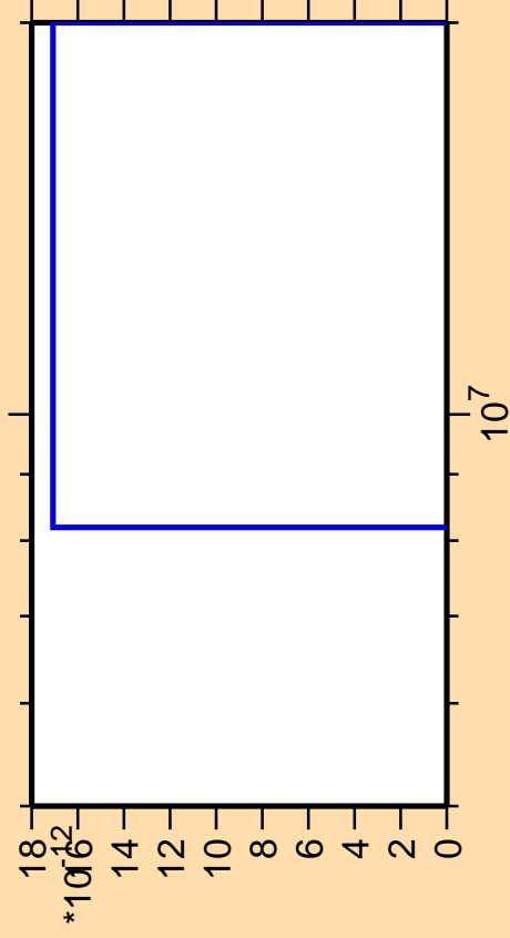
\Delta\sigma/\sigma vs. E for ^{151}\text{Ho} (mt 42)
