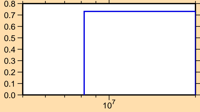
\sigma vs. E for ^{151}\text{Ho}(n,2n)
