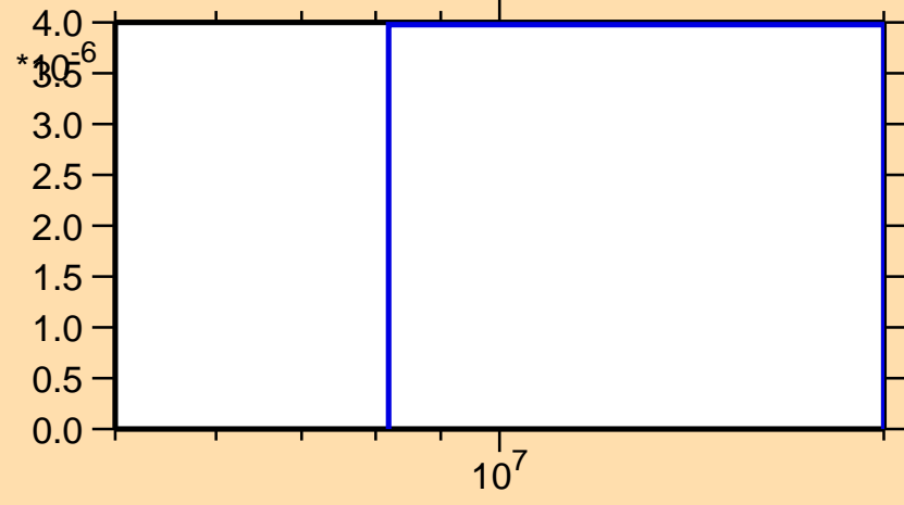
\sigma vs. E for ^{151}\text{Ho}(n,\text{nd})
