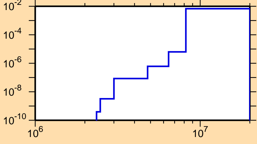
\sigma vs. E for ^{151}\text{Ho}(n,d)
