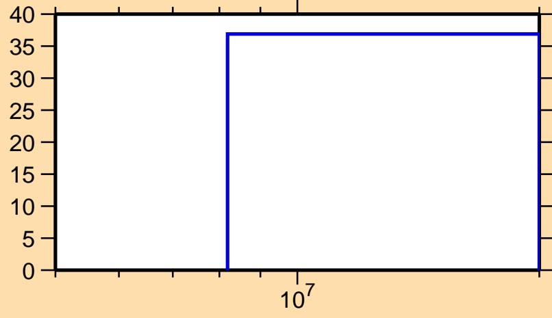
\Delta\sigma/\sigma vs. E for ^{151}\text{Ho}(n,\text{el.})
