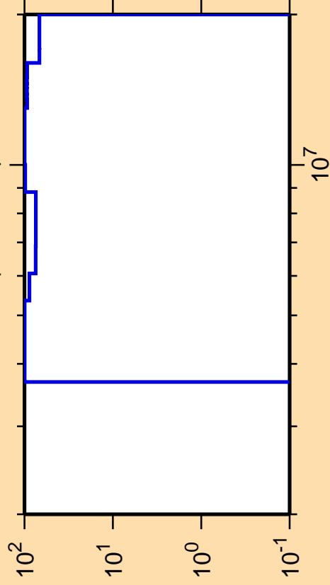
\Delta\sigma/\sigma vs. E for ^{152}\text{Ho}(n,\text{ncont.})
