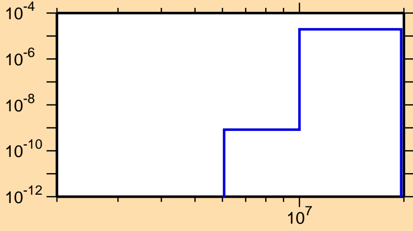
\sigma vs. E for ^{152}\text{Ho} (mt 45)
