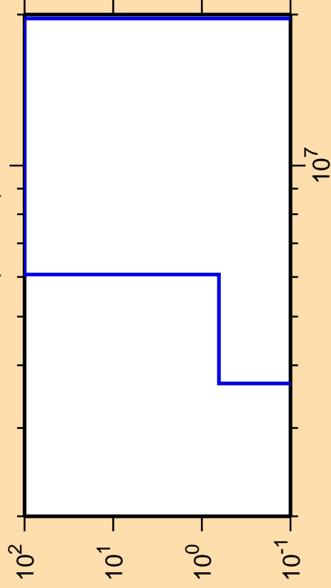
\Delta\sigma/\sigma vs. E for ^{152}\text{Ho} (mt 45)
