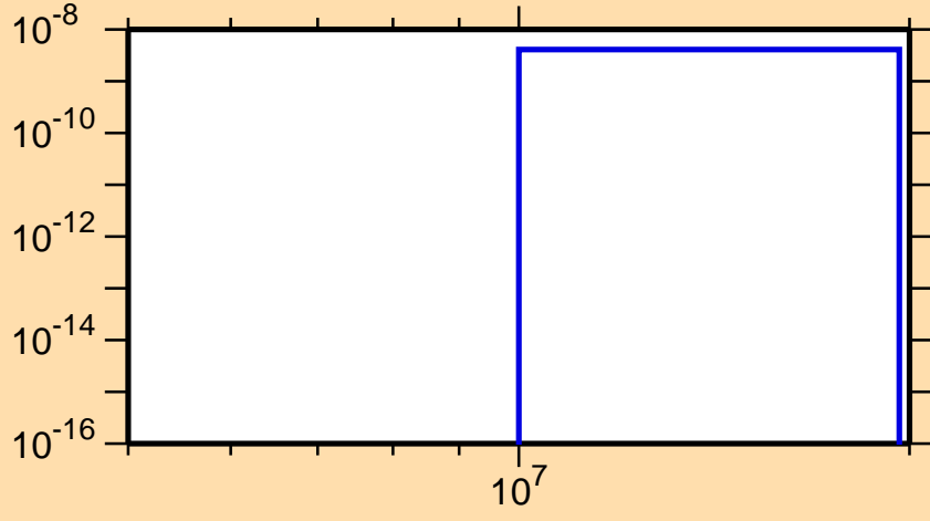
\sigma vs. E for ^{152}\text{Ho}(n,\text{pd})
