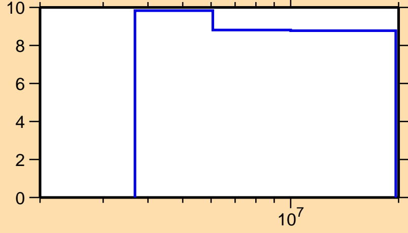
\Delta\sigma/\sigma vs. E for ^{152}\text{Ho}(n,n\text{onel.})
