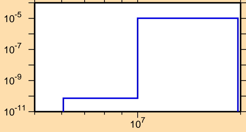
\sigma vs. E for ^{152}\text{Ho}(n,\text{He3})
