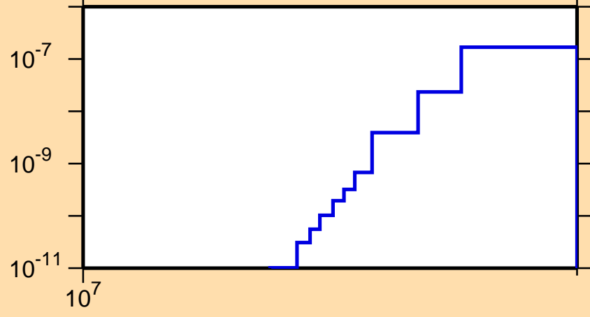
\sigma vs. E for ^{152}\text{Ho}(n,\text{pd})
