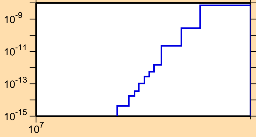
\sigma vs. E for ^{152}\text{Ho} (mt 34)
