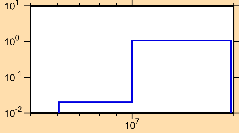
\sigma vs. E for ^{152}\text{Ho}(n,2n)
