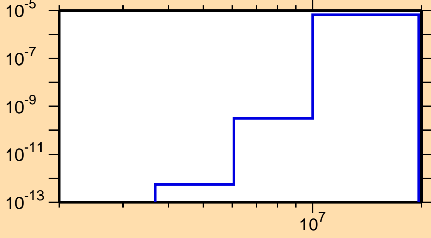
\sigma vs. E for ^{152}\text{Ho} (mt 45)
