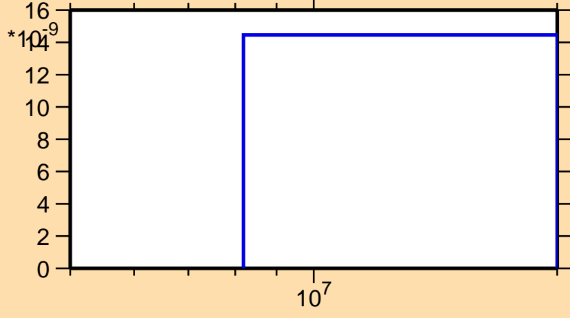
\sigma vs. E for ^{152}\text{Ho}(n,\text{nt})
