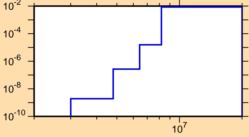
\sigma vs. E for ^{152}\text{Ho}(n,d)
