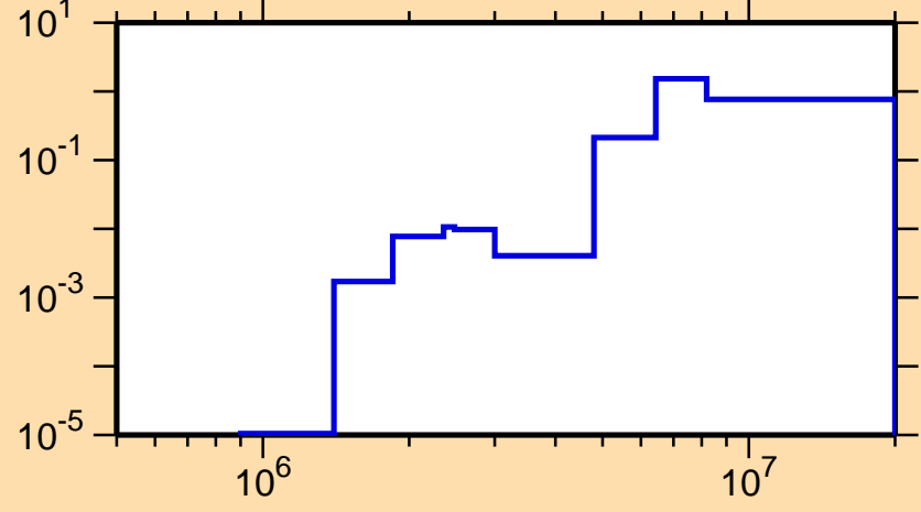
\sigma vs. E for ^{152}\text{Ho}(n,n\text{cont.})
