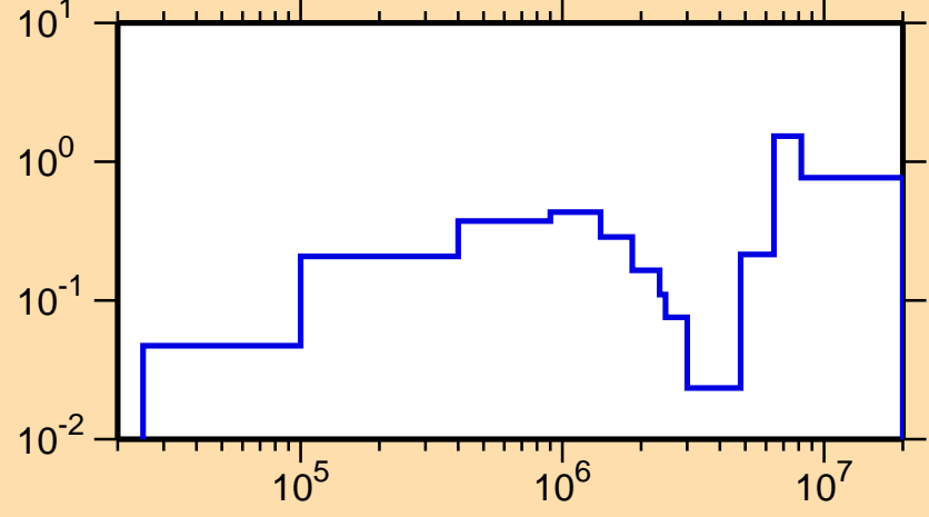
\sigma vs. E for ^{152}\text{Ho}(n,\text{inel.})
