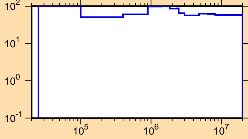
\Delta\sigma/\sigma vs. E for ^{153}\text{Ho}(n,n_1)
