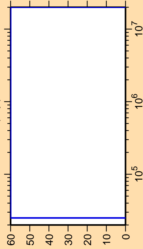
\Delta\sigma/\sigma vs. E for ^{153}\text{Ho}(n,p)
