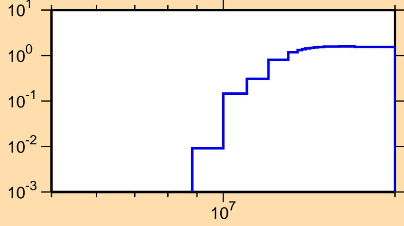
\sigma vs. E for ^{153}\text{Ho}(n,2n)
