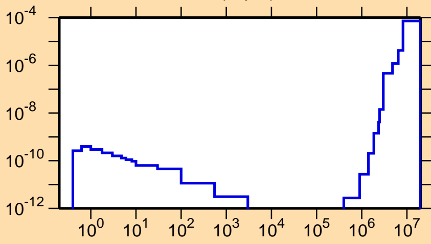
\sigma vs. E for ^{153}\text{Ho}(n,p\alpha)
