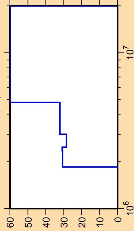
\Delta\sigma/\sigma vs. E for ^{153}\text{Ho}(n,\gamma)
