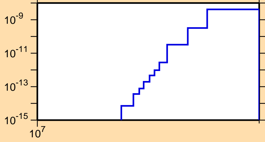
\sigma vs. E for ^{154}\text{Ho}(n,\text{pd})
